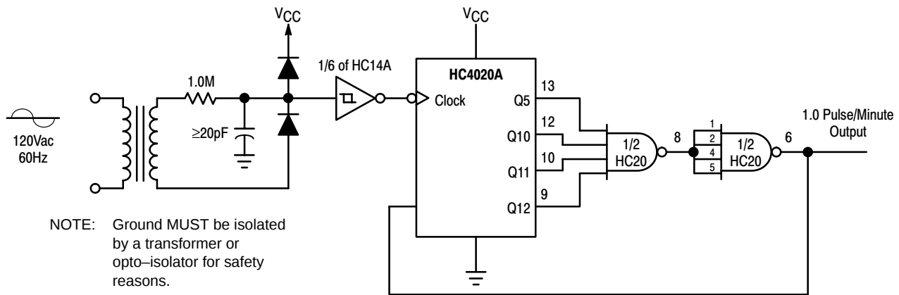
Figure 7. Time-Base Generator
