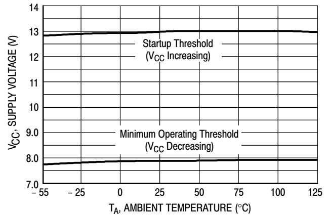
Figure 15. Undervoltage Lockout Thresholds versus Temperature
