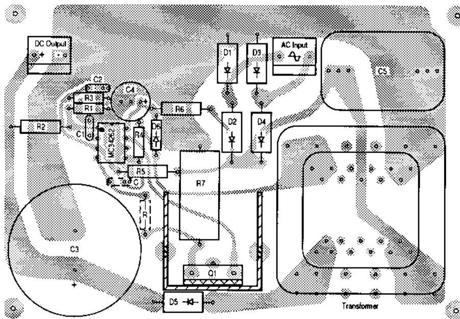
Figure 29. Printed Circuit Board and Component Layout (Circuits of Figures 15 and 16)
