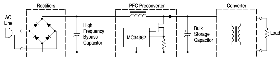
Figure 18. Active Power Factor Correction Preconverter
