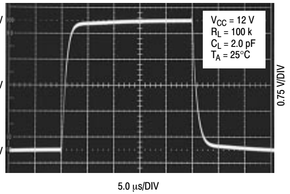
Figure 7. Error Amp Transient Response
