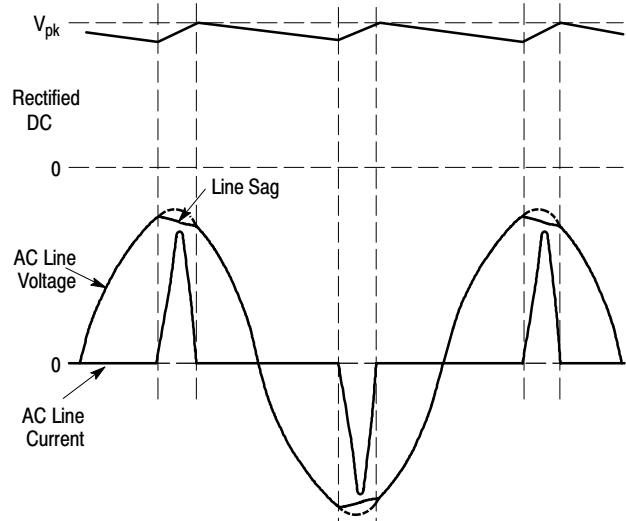
Figure 17. Uncorrected Power Factor Input Waveforms
