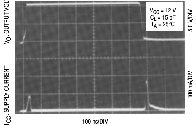
Figure 13. Drive Output Cross Conduction
