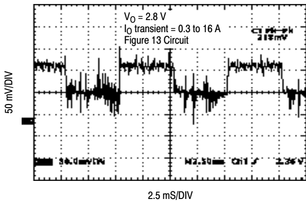
Figure 5. Feedback Circuit Load Transient Response
