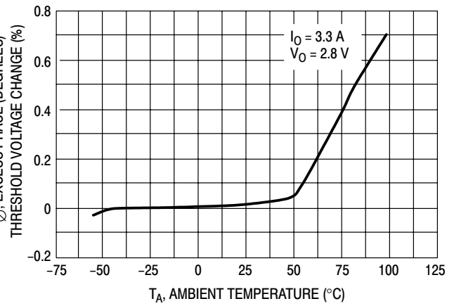
Figure 8. Feedback Threshold Voltage versus Temperature
