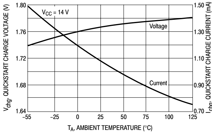
Figure 8. Quickstart Charge Current versus Temperature
