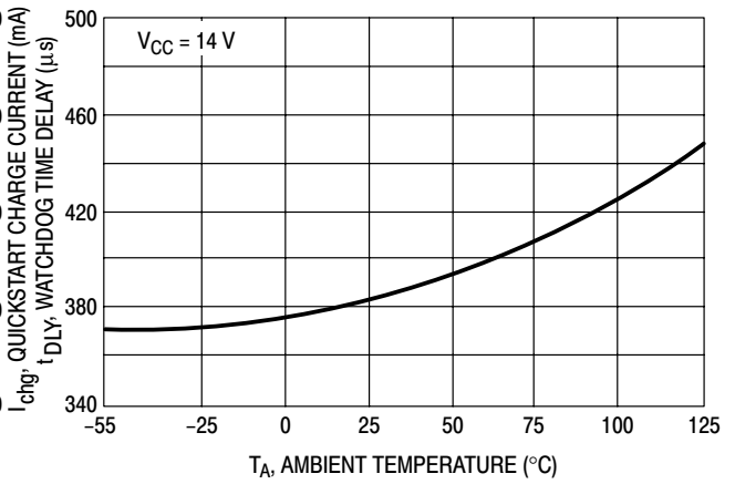
Figure 9. Watchdog Timer Delay versus Temperature
