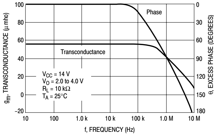
Figure 6. Error Amplifier Transconductance and Phase versus Frequency
