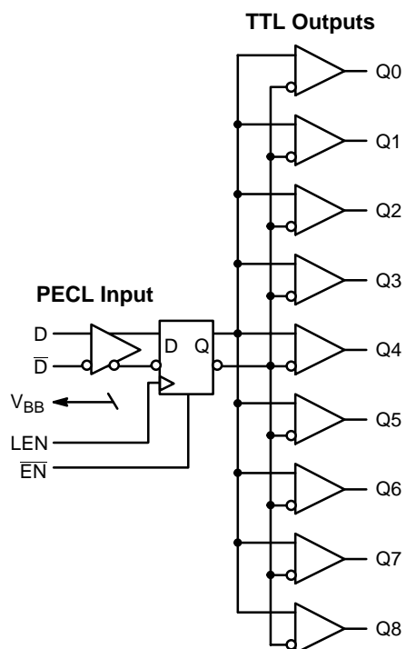
Figure 2. Logic Diagram
