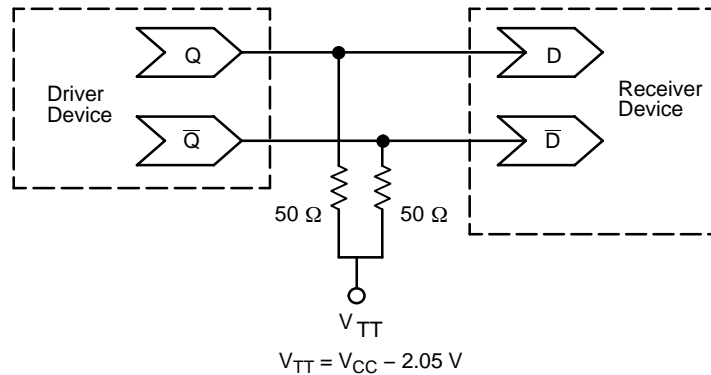
Figure 7. Typical Termination for Output Driver and Device Evaluation (See Application Note AND8020 – Termination of ECL Logic Devices.)
