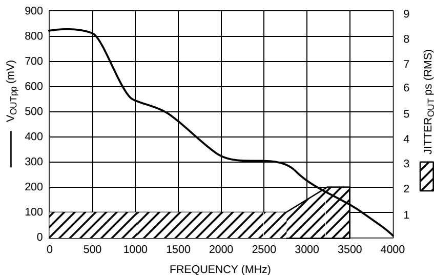
Figure 3. F_{\max}/\text{Jitter} for \overline{Q} Output
