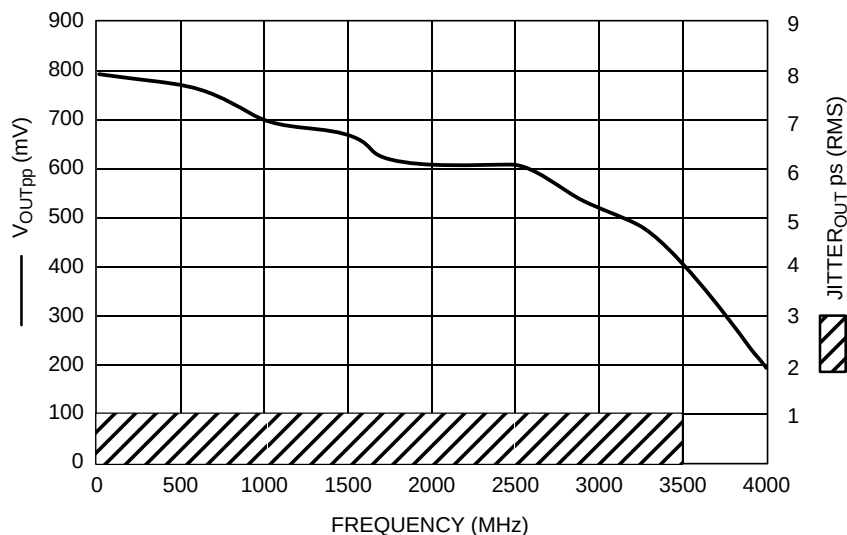
Figure 2. F_{\max}/\text{Jitter} for QHG, \overline{QHG} Output
