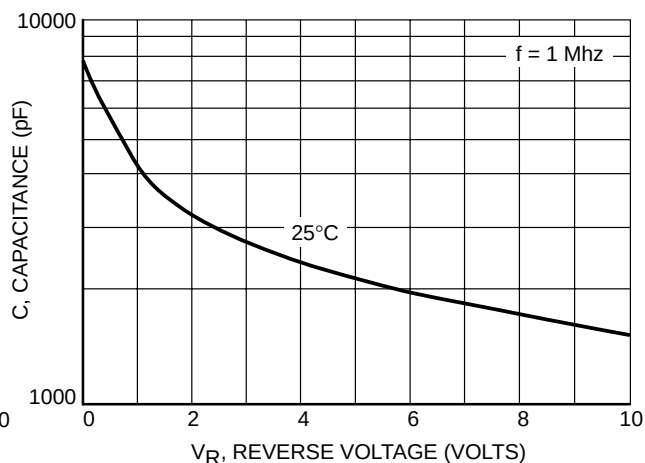
Figure 4. Typical Capacitance
