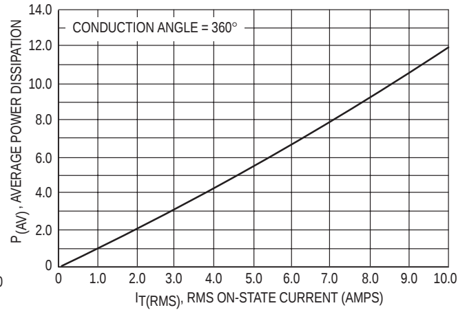
Figure 2. Power Dissipation
