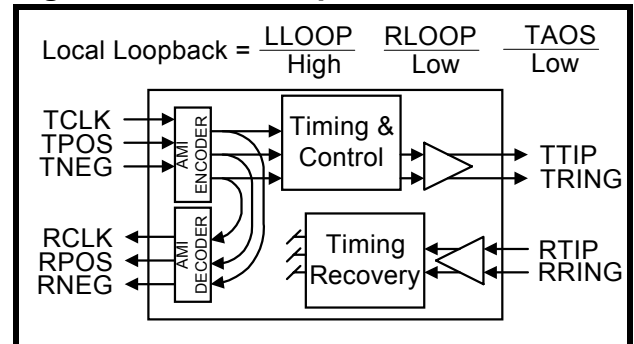
Figure 8: Local Loopback
