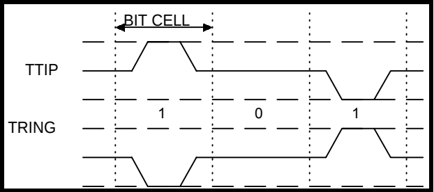
Figure 2: 50% AMI Coding
