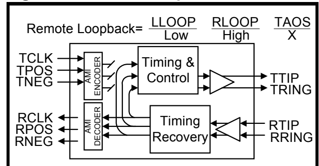
Figure 9: Remote Loopback
