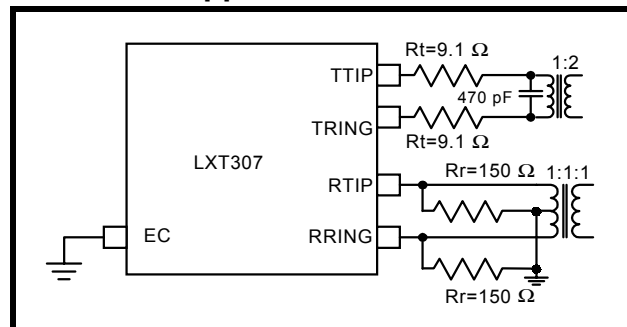
Figure 11: Line Interface for E1 Coax Applications
