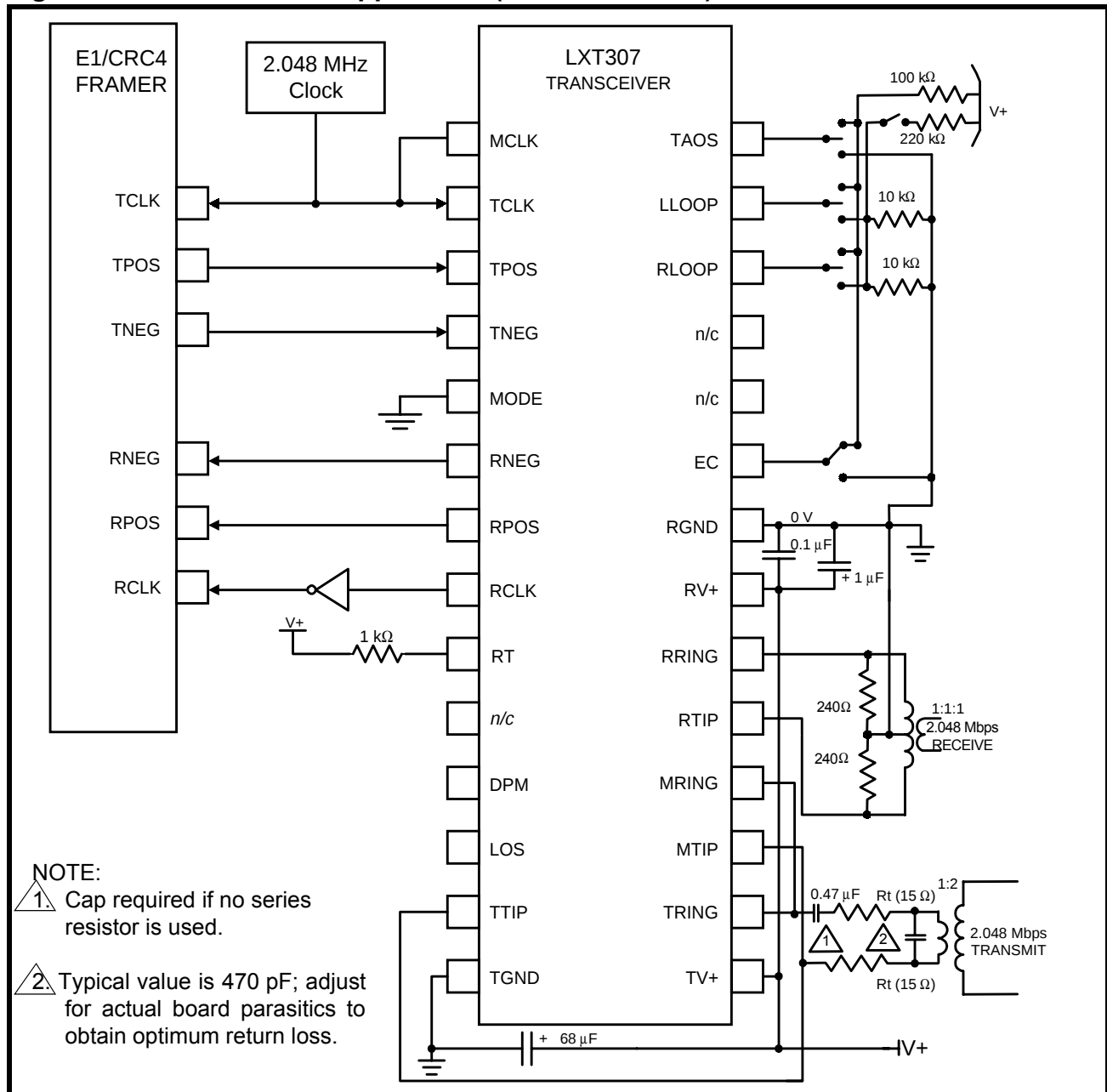
Figure 10: LXT307 120 \Omega Application (Hardware Mode)
