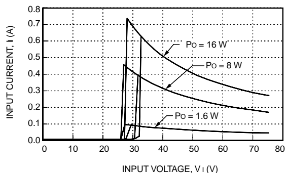
Figure 1. LW016AJ, BK, CL Typical Input Characteristics
