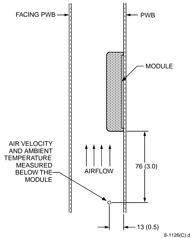
Figure 16. Experimental Test Setup
