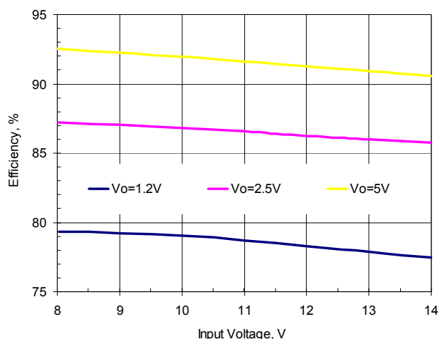
Figure 4. Efficiency vs. Input Voltage. Iout=10A, Fsw=500kHz
