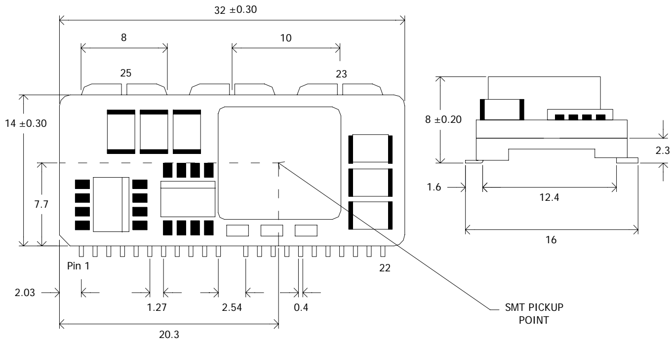
Figure 58. Mechanical Drawing
