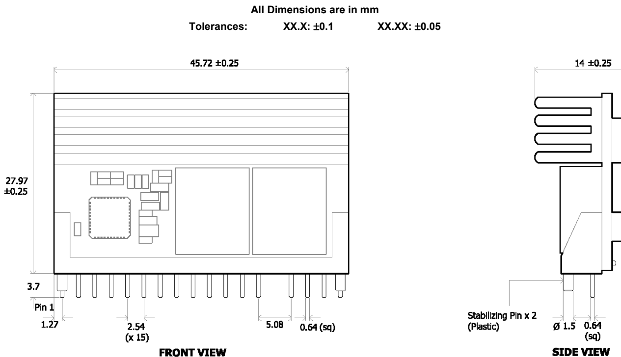
Figure 14. Mechanical Drawing
