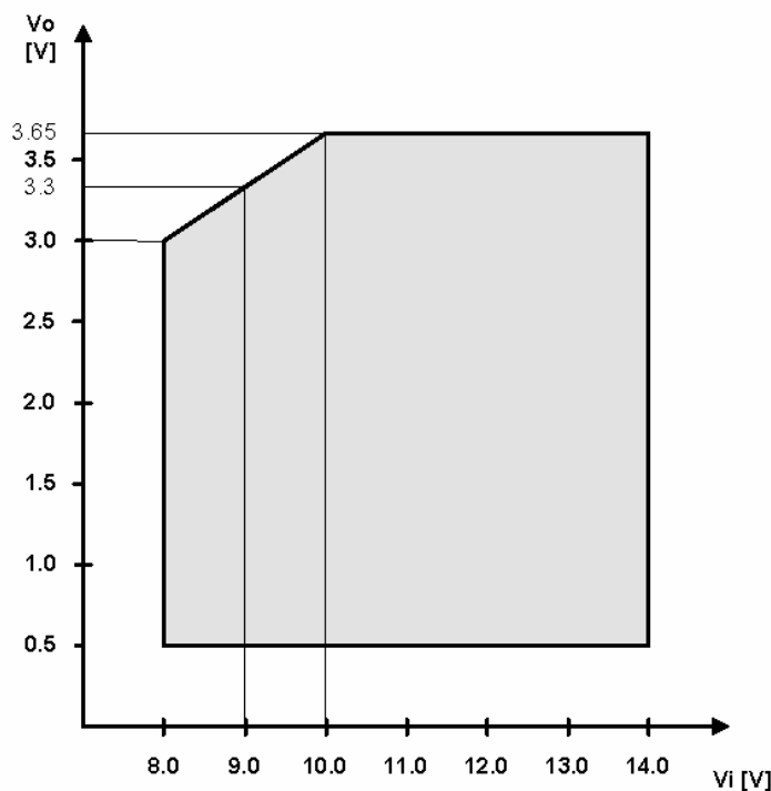
Figure 1. Output Voltage as a Function of Input Voltage
