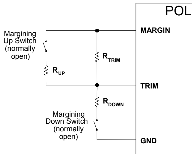
Figure 14. Alternative Margining Configuration
