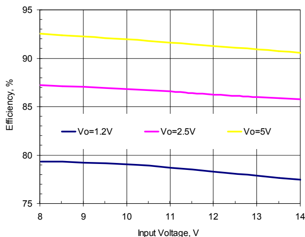
Figure 4. Efficiency vs. Input Voltage. Iout=10A
