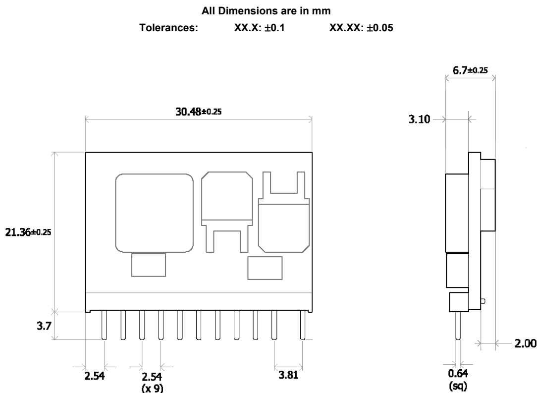
Figure 15. Mechanical Drawing
