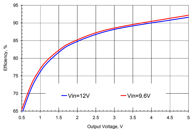
Figure 3. Efficiency vs. Output Voltage, Iout=10A
