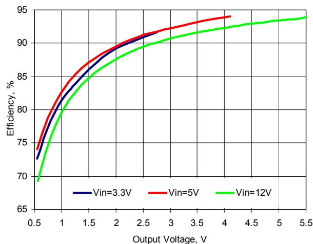
Figure 5. Efficiency vs. Output Voltage, Iout=15A
