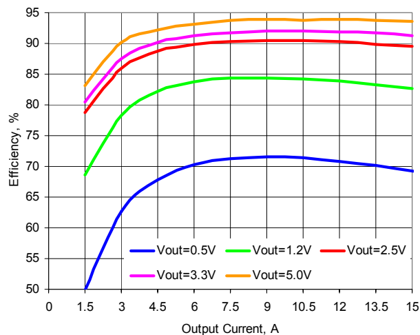
Figure 4. Efficiency vs. Load. Vin=12V
