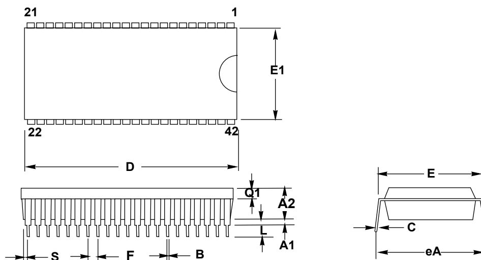
Figure 23 42-Lead Shrink Dual-in-line Package (SDIP)
