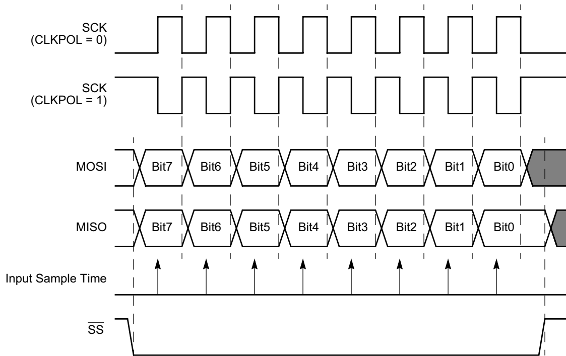
Figure 34. ESPI Timing when \text{PHASE} = 0
