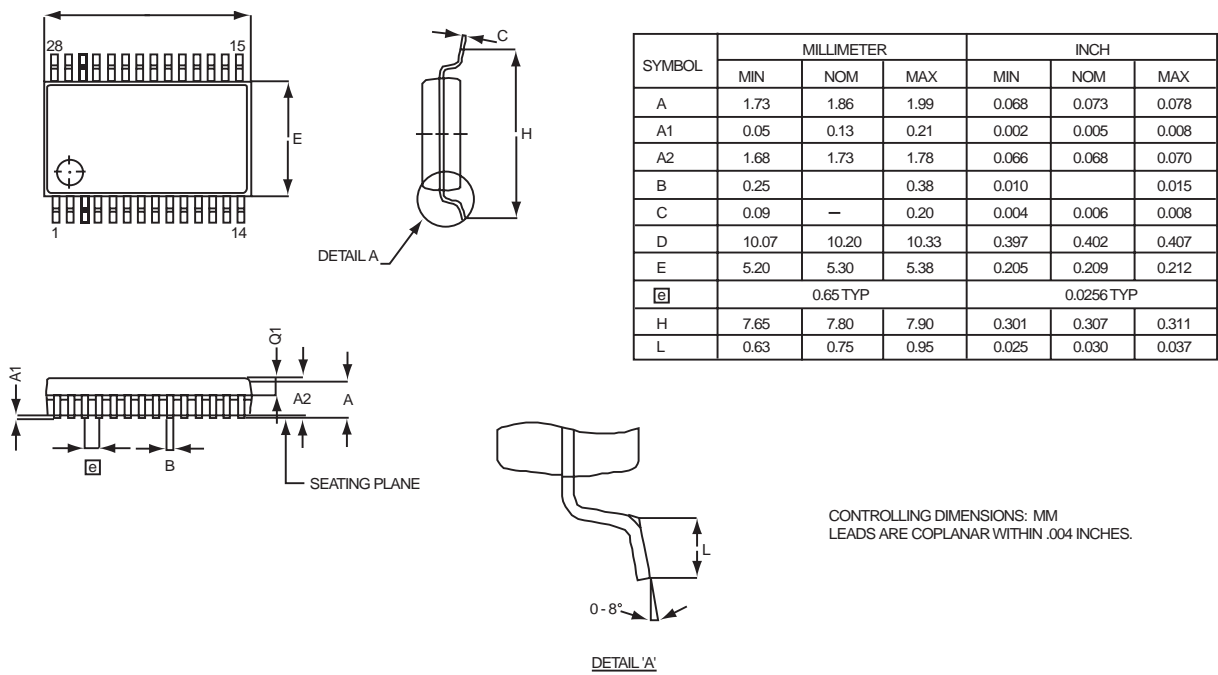
Figure 85 displays the 28-pin Small Shrink Outline Package (SSOP) available for the Z8 Encore! XP F1680 Series devices.
