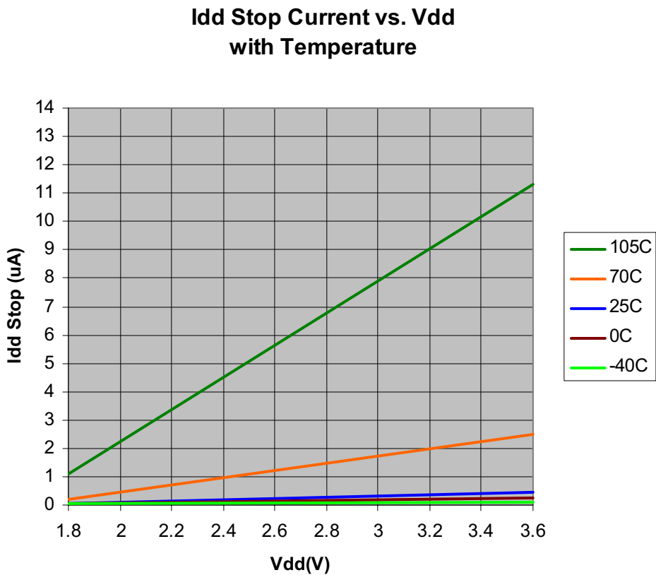
Figure 73. STOP Mode Current Consumption as a Function Vdd with Temperature as a Parameter— All Peripheral Disabled
