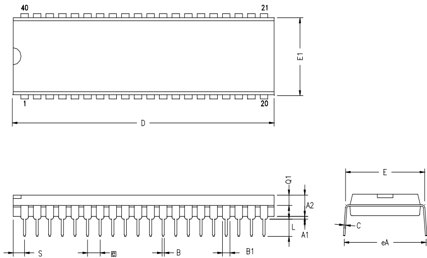
Figure 86. 40-Lead Plastic Dual-Inline Package (PDIP)
