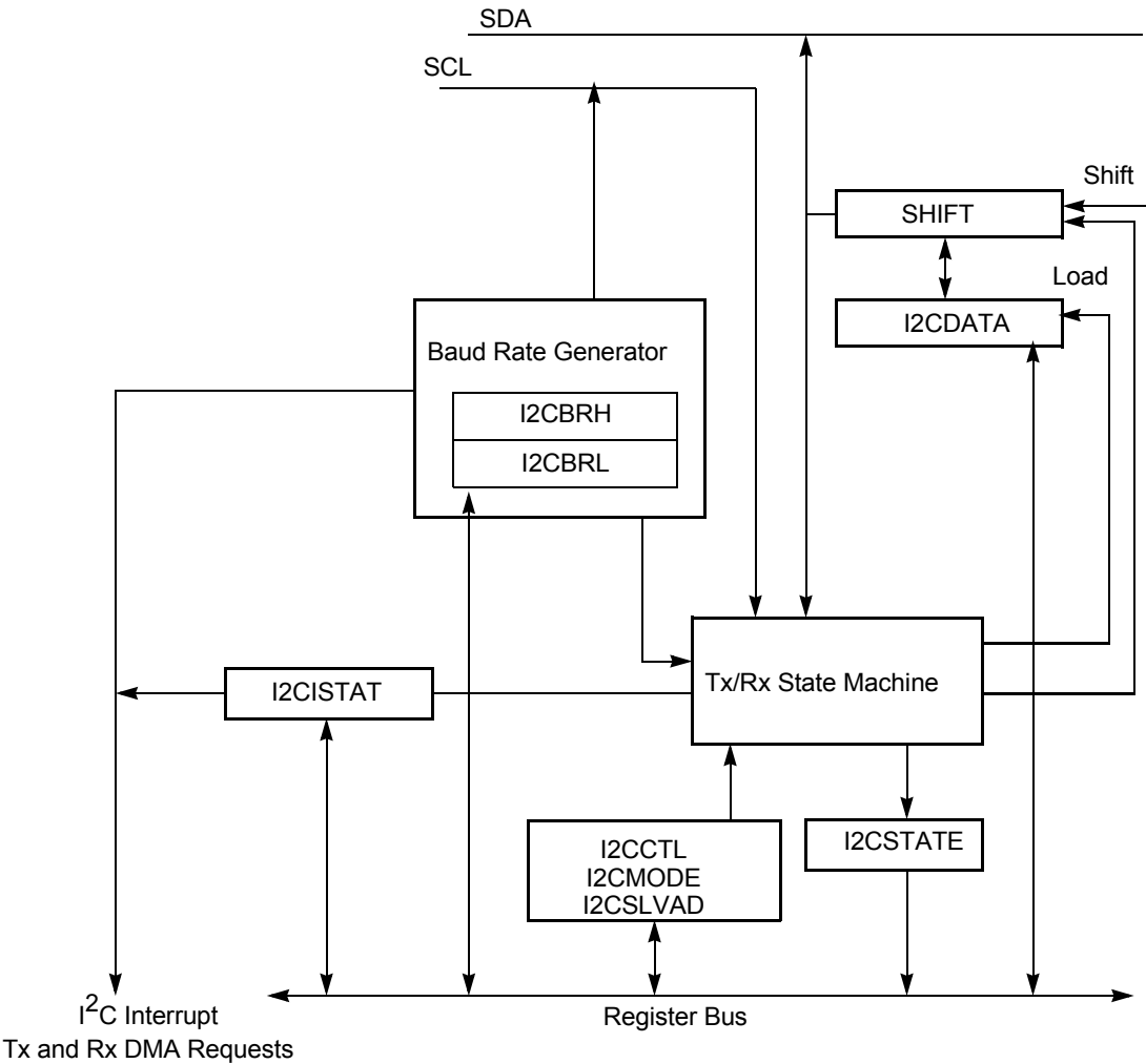
Figure 42 illustrates the architecture of the I 2 C Controller.
