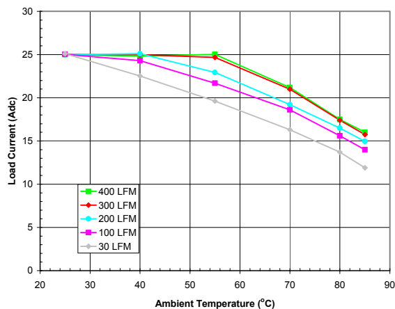
Fig. 15: Available load current vs. ambient temperature and airflow rates for V out = 1.8 V with V in = 12 V, and maximum MOSFET temperature ≤ 110 °C. Horizontal Orientation (Airflow from Vin pin to GND pin.)
