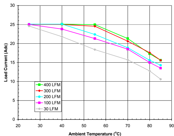
Fig. 14: Available load current vs. ambient temperature and airflow rates for V out = 3.3 V with V in = 12 V, and maximum MOSFET temperature ≤ 110 °C. Horizontal Orientation (Airflow from Vin pin to GND pin.)
