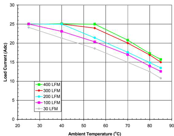
Fig. 13: Available load current vs. ambient temperature and airflow rates for V out = 5.0 V with V in = 12 V, and maximum MOSFET temperature ≤ 110 °C. Horizontal Orientation (Airflow from Vin pin to GND pin.)
