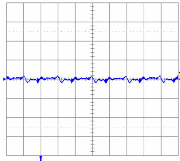
Fig. 22: Output voltage ripple (20 mV/div.) at full rated load current into a resistive load with external capacitance 1 µF ceramic and V_{in} = 12 V for V_{out} = 1.2 V. Time Scale: 1 µs/div.
