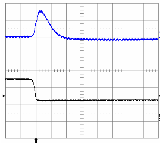
Fig. 24: Output voltage response for V_{out} = 3.3 V to negative load current step change from 25 A to 12.5 A with slew rate of -5 A/µs at V_{in} = 12 V. Top Trace: Output Voltage (100 mV/div.); Bottom Trace: Load Current (10 A/div.) C_o = 1 µF ceramic. Time Scale: 10 µs/div.
