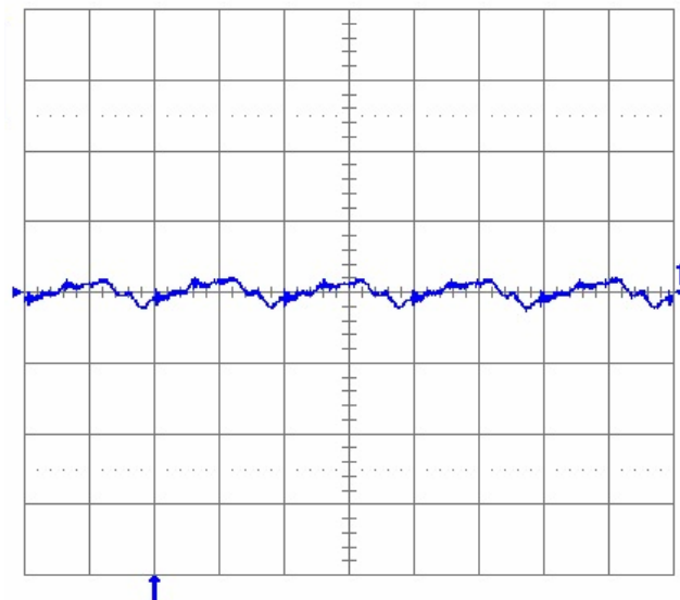
Fig. 21: Output voltage ripple (20 mV/div.) at full rated load current into a resistive load with external capacitance 1 µF ceramic and V_{in} = 12 V for V_{out} = 3.3 V. Time Scale: 1 µs/div.
