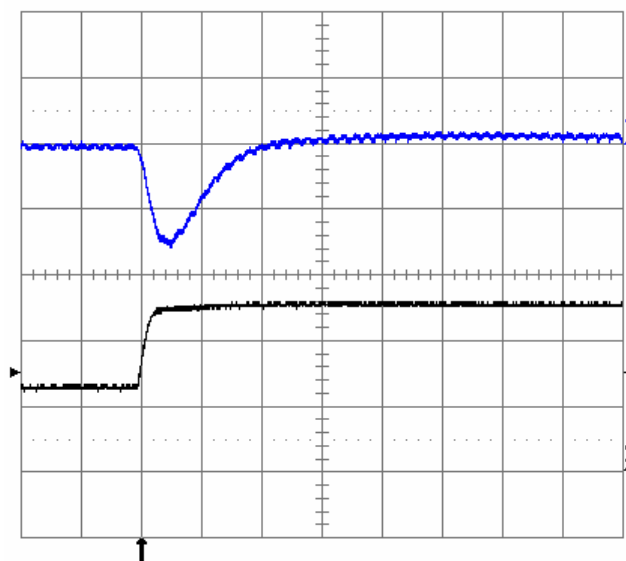
Fig. 23: Output voltage response for V_{out} = 3.3 V to positive load current step change from 12.5 A to 25 A with slew rate of 5 A/µs at V_{in} = 12 V. Top Trace: Output Voltage (100 mV/div.); Bottom Trace: Load Current (10 A/div.) C_o = 1 µF ceramic. Time Scale: 10 µs/div.
