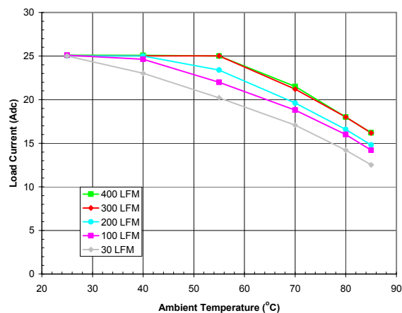
Fig. 16: Available load current vs. ambient temperature and airflow rates for V out = 1.2 V with V in = 12 V, and maximum MOSFET temperature ≤ 110 °C. Horizontal Orientation (Airflow from Vin pin to GND pin.)
