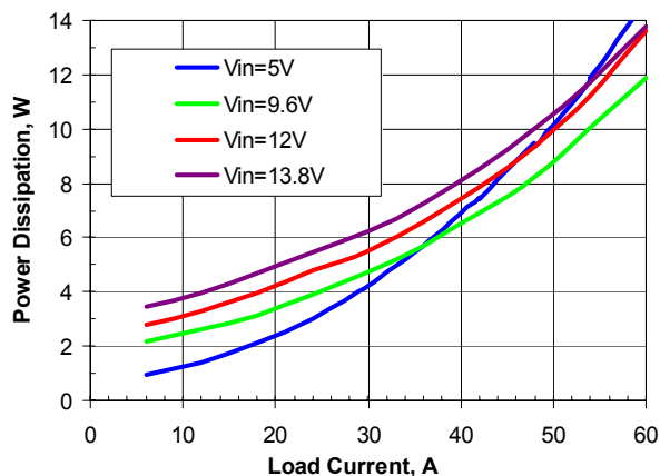
Figure 12. Power Dissipation vs. Load. Vout=2.5V
