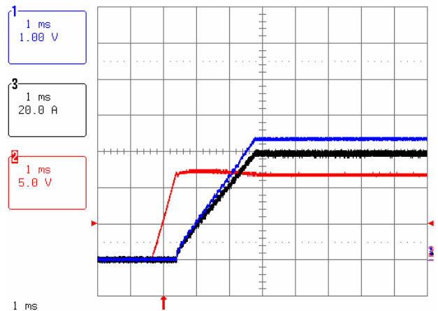
Figure 17. Typical Start-Up with application of Vin ( V_o = 3.3\text{Vdc} , I_o = 60\text{A} ). Ch1 – Vout, Ch2 – Vin, Ch3 – Iout
