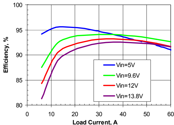
Figure 6. Efficiency vs. Load. Vout=2.5V
