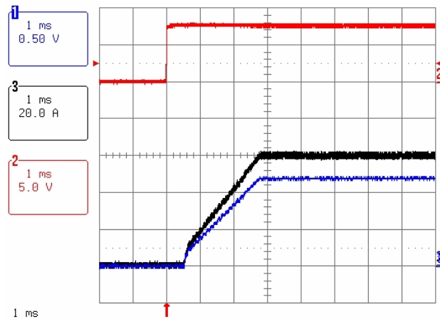
Figure 14. Typical Start-Up Using Remote On/Off ( V_o = 1.2\text{Vdc} , I_o=60\text{A} ). Ch1 – Vout, Ch2 – On/Off, Ch3 – Iout
