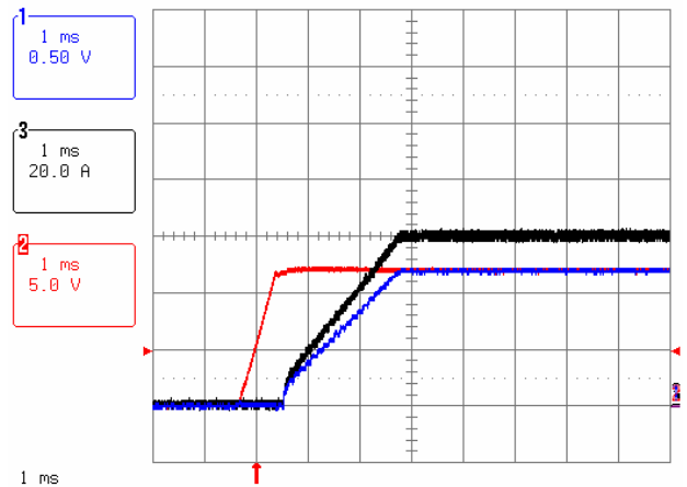
Figure 16. Typical Start-Up with application of Vin ( V_o = 1.2\text{Vdc} , I_o = 60\text{A} ). Ch1 – Vout, Ch2 – Vin, Ch3 – Iout
