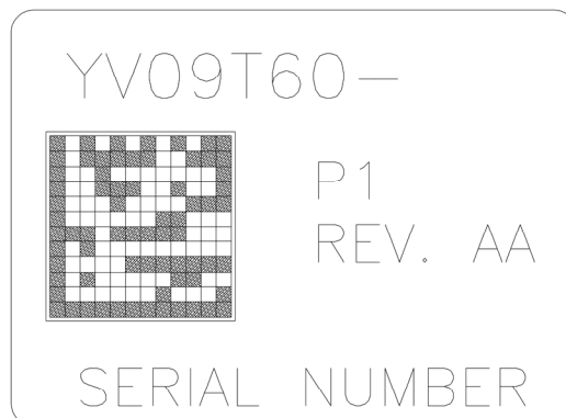
Figure 1. Label Drawing
