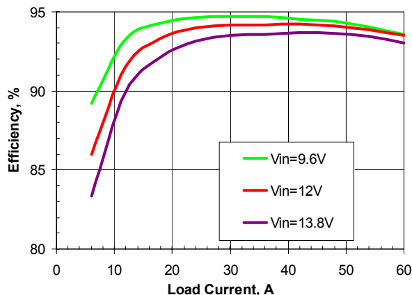
Figure 7. Efficiency vs. Load. Vout=3.3V
