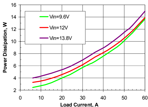
Figure 13. Power Dissipation vs. Load. Vout=3.3V
