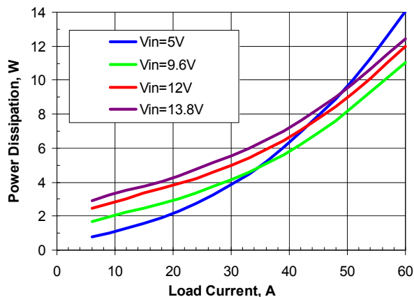
Figure 11. Power Dissipation vs. Load. Vout=1.8V
