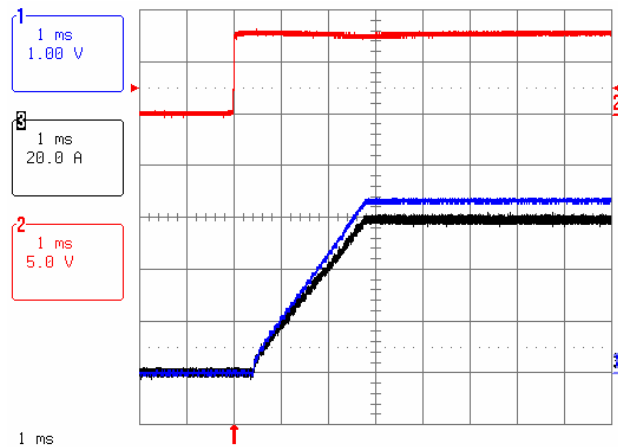
Figure 15. Typical Start-Up Using Remote On/Off ( V_o = 3.3\text{Vdc} , I_o=60\text{A} ). Ch1 – Vout, Ch2 – On/Off, Ch3 – Iout
