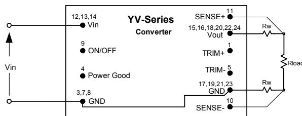
Figure 28. Remote Sense Circuit Configuration
