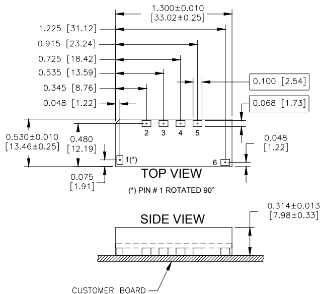
YS12S Pinout (Surface Mount)
