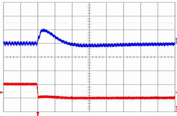
Fig. 1.2V.8: Output voltage response for V_{out} = 1.2 V to negative load current step change from 10 A to 5 A with slew rate of -5 A/ \mu s at V_{in} = 12 V. Top trace: output voltage (100 mV/div.); Bottom trace: load current (5 A/div.). C_o = 100 \mu F ceramic. Time scale: 20 \mu s/div.
