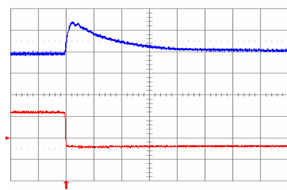
Fig. 1.8V.8: Output voltage response for V_{out} = 1.8 V to negative load current step change from 16 A to 8 A with slew rate of -5 A/ \mu s at V_{in} = 5 V. Top trace: output voltage (100 mV/div.); Bottom trace: load current (5 A/div.). C_o = 100 \mu F ceramic. Time scale: 20 \mu s/div.
