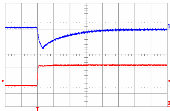
Fig. 1.8V.7: Output voltage response for V_{out} = 1.8 V to positive load current step change from 8 A to 16 A with slew rate of 5 A/ \mu s at V_{in} = 5 V. Top trace: output voltage (100 mV/div.); Bottom trace: load current (5 A/div.). C_o = 100 \mu F ceramic. Time scale: 20 \mu s/div.
