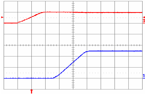
Fig. 2.5V.5: Turn-on transient for V_{out} = 2.5 V with application of V_{in} at full rated load current (resistive) and 100\text{ }\mu\text{F} external capacitance at V_{in} = 5 V. Top trace: V_{in} (5 V/div.); Bottom trace: output voltage (1 V/div.); Time scale: 2 ms/div.
