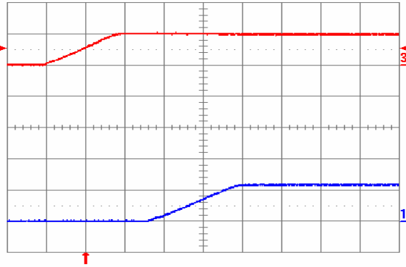
Fig. 1.2V.5: Turn-on transient for V_{out} = 1.2 V with application of V_{in} at full rated load current (resistive) and 100 \mu F external capacitance at V_{in} = 5 V. Top trace: V_{in} (5 V/div.); Bottom trace: output voltage (1 V/div.); Time scale: 2 ms/div.
