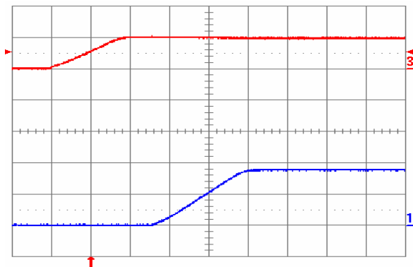
Fig. 1.8V.5: Turn-on transient for V_{out} = 1.8 V with application of V_{in} at full rated load current (resistive) and 100 \mu F external capacitance at V_{in} = 5 V. Top trace: V_{in} (5 V/div.); Bottom trace: output voltage (1V/div.); Time scale: 2 ms/div.
