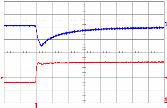
Fig. 0.7525V.7: Output voltage response for V_{out} = 0.7525 V to positive load current step change from 8 A to 16 A with slew rate of 5 A/ \mu\text{s} at V_{in} = 5 V. Top trace: output voltage (100 mV/div.); Bottom trace: load current (5 A/div.). C_o = 100\ \mu\text{F} ceramic. Time scale: 20 \mu\text{s} /div.
