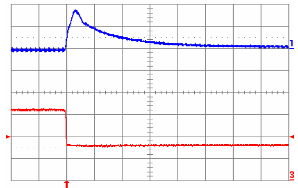
Fig. 0.7525V.8: Output voltage response for V_{out} = 0.7525 V to negative load current step change from 16 A to 8 A with slew rate of -5 A/ \mu\text{s} at V_{in} = 5 V. Top trace: output voltage (100 mV/div.); Bottom trace: load current (5 A/div.). C_o = 100\ \mu\text{F} ceramic. Time scale: 20 \mu\text{s} /div.
