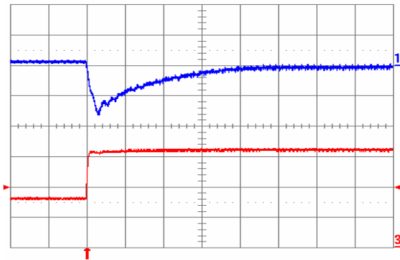
Fig. 2.5V.7: Output voltage response for V_{out} = 2.5 V to positive load current step change from 8 A to 16 A with slew rate of 5\text{ A}/\mu\text{s} at V_{in} = 5 V. Top trace: output voltage (100 mV/div.); Bottom trace: load current (5 A/div.). C_o = 100\text{ }\mu\text{F} ceramic. Time scale: 20 \mu\text{s} /div.
