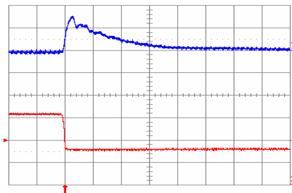
Fig. 3.3V.8: Output voltage response for V_{out} = 3.3 V to negative load current step change from 16 A to 8 A with slew rate of -5 A/ \mu s at V_{in} = 5 V. Top trace: output voltage (100 mV/div.); Bottom trace: load current (5 A/div.). C_o = 100 \mu F ceramic. Time scale: 20 \mu s/div.
