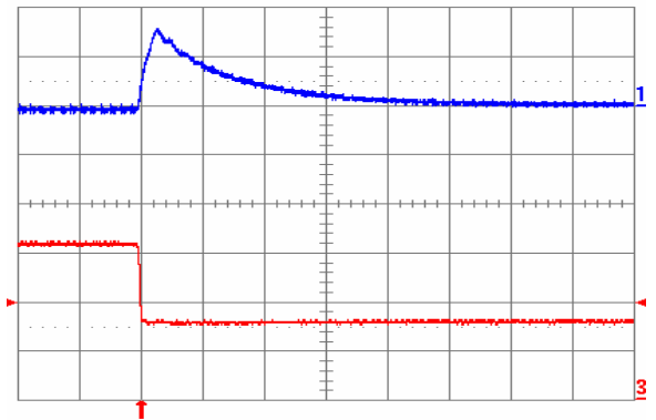
Fig. 1.2V.8: Output voltage response for V_{out} = 1.2 V to negative load current step change from 16 A to 8 A with slew rate of -5 A/ \mu s at V_{in} = 5 V. Top trace: output voltage (100 mV/div.); Bottom trace: load current (5 A/div.). C_o = 100 \mu F ceramic. Time scale: 20 \mu s/div.
