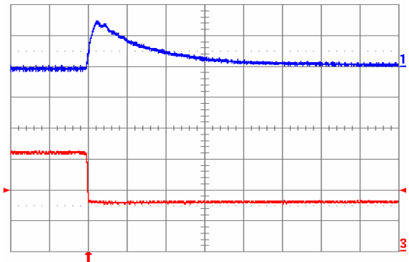
Fig. 1.5V.8: Output voltage response for V_{out} = 1.5 V to negative load current step change from 16 A to 8 A with slew rate of -5 A/ \mu s at V_{in} = 5 V. Top trace: output voltage (100 mV/div.); Bottom trace: load current (5 A/div.). C_o = 100 \mu F ceramic. Time scale: 20 \mu s/div.
