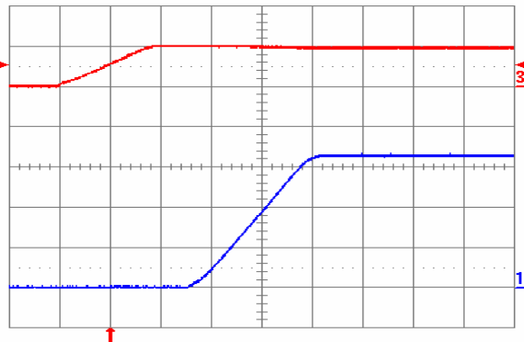
Fig. 3.3V.5: Turn-on transient for V_{out} = 3.3 V with application of V_{in} at full rated load current (resistive) and 100 \mu F external capacitance at V_{in} = 5 V. Top trace: V_{in} (5 V/div.); Bottom trace: output voltage (1 V/div.); Time scale: 2 ms/div.
