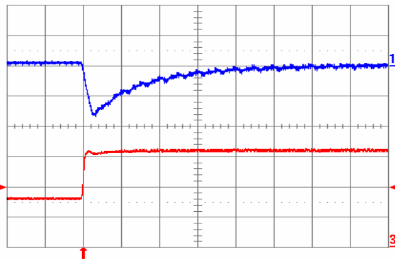
Fig. 1.2V.7: Output voltage response for V_{out} = 1.2 V to positive load current step change from 8 A to 16 A with slew rate of 5 A/ \mu s at V_{in} = 5 V. Top trace: output voltage (100 mV/div.); Bottom trace: load current (5 A/div.). C_o = 100 \mu F ceramic. Time scale: 20 \mu s/div.
