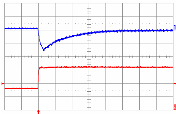
Fig. 2.0V.7: Output voltage response for V_{out} = 2.0 V to positive load current step change from 8 A to 16 A with slew rate of 5 A/ \mu s at V_{in} = 5 V. Top trace: output voltage (100 mV/div.); Bottom trace: load current (5 A/div.). C_o = 100 \mu F ceramic. Time scale: 20 \mu s/div.
