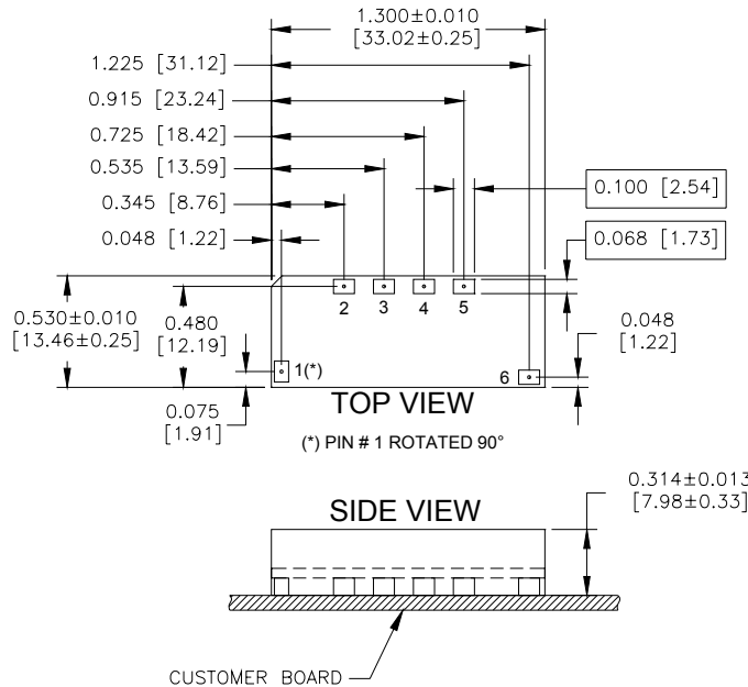
YS05S Pinout (Surface-Mount)
