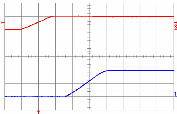
Fig. 2.0V.5: Turn-on transient for V_{out} = 2.0 V with application of V_{in} at full rated load current (resistive) and 100 \mu F external capacitance at V_{in} = 5 V. Top trace: V_{in} (5 V/div.); Bottom trace: output voltage (1 V/div.); Time scale: 2 ms/div.
