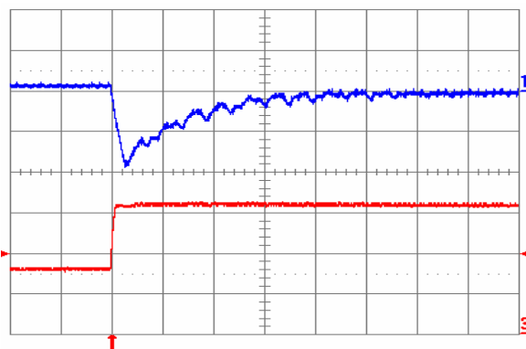
Fig. 3.3V.7: Output voltage for V_{out} = 3.3 V to positive load current step change from 8 A to 16 A with slew rate of 5 A/ \mu s at V_{in} = 5 V. Top trace: output voltage (100 mV/div.); Bottom trace: load current (5 A/div.). C_o = 100 \mu F ceramic. Time scale: 20 \mu s/div.
