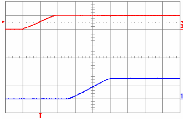
Fig. 1.5V.5: Turn-on transient for V_{out} = 1.5 V with application of V_{in} at full rated load current (resistive) and 100 \mu F external capacitance at V_{in} = 5 V. Top trace: V_{in} (5 V/div.); Bottom trace: output voltage (1 V/div.); Time scale: 2 ms/div.
