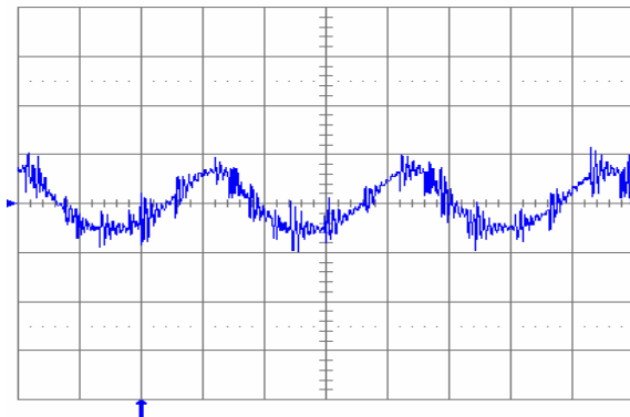
Fig. 3.3V.6: Output voltage ripple (20 mV/div.) at full rated load current into a resistive load with external capacitance 100 \mu F ceramic + 1 \mu F ceramic and V_{in} = 5 V for V_{out} = 3.3 V. Time scale: 2 \mu s/div.
