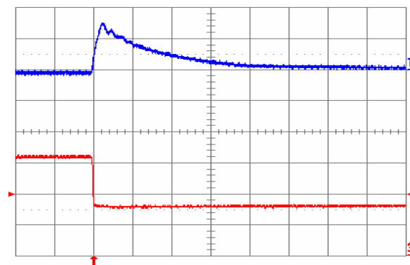
Fig. 2.0V.8: Output voltage response for V_{out} = 2.0 V to negative load current step change from 16 A to 8 A with slew rate of -5 A/ \mu s at V_{in} = 5 V. Top trace: output voltage (100 mV/div.); Bottom trace: load current (5 A/div.). C_o = 100 \mu F ceramic. Time scale: 20 \mu s/div.
