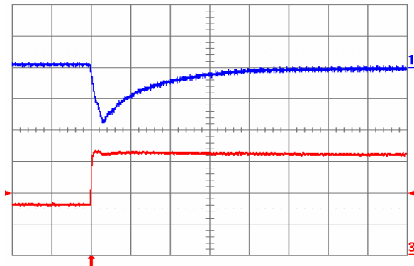
Fig. 1.5V.7: Output voltage response for V_{out} = 1.5 V to positive load current step change from 8 A to 16 A with slew rate of 5 A/ \mu s at V_{in} = 5 V. Top trace: output voltage (100 mV/div.); Bottom trace: load current (5 A/div.). C_o = 100 \mu F ceramic. Time scale: 20 \mu s/div.
