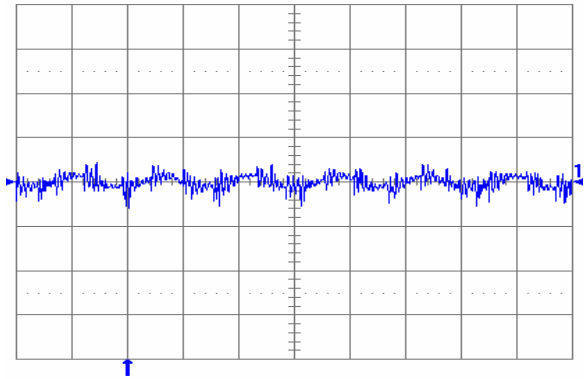
Fig. 1.5V.6: Output voltage ripple (20 mV/div.) at full rated load current into a resistive load with external capacitance 100 \mu F ceramic + 1 \mu F ceramic and V_{in} = 5 V for V_{out} = 1.5 V. Time scale: 2 \mu s/div.
