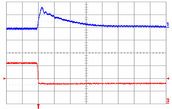
Fig. 2.5V.8: Output voltage response for V_{out} = 2.5 V to negative load current step change from 16 A to 8 A with slew rate of -5\text{ A}/\mu\text{s} at V_{in} = 5 V. Top trace: output voltage (100 mV/div.); Bottom trace: load current (5 A/div.). C_o = 100\text{ }\mu\text{F} ceramic. Time scale: 20 \mu\text{s} /div.
