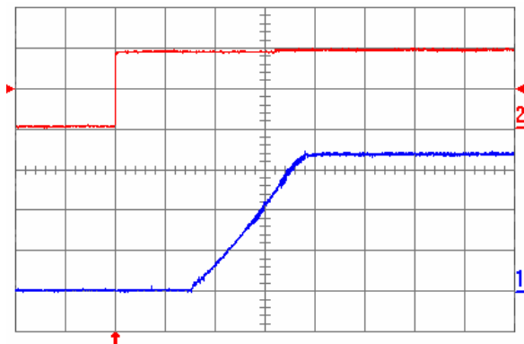
Fig. 0.7525V.5: Turn-on transient for V_{out} = 0.7525 V with the application of Enable signal at full rated load current (resistive) and 100\text{ }\mu\text{F} external capacitance at V_{in} = 5 V. Top trace: Enable signal (2 V/div.); Bottom trace: output voltage (200 mV/div.); Time scale: 2 ms/div.
