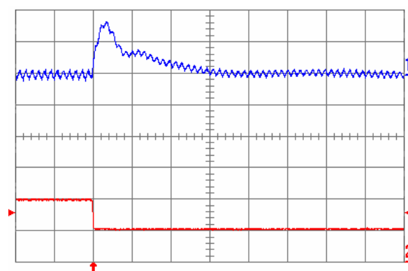
Fig. 2.0V.8: Output voltage response for V_{out} = 2.0 V to negative load current step change from 10 A to 5 A with slew rate of -5 A/ \mu s at V_{in} = 5 V. Top trace: output voltage (100 mV/div.); Bottom trace: load current (5 A/div.). C_o = 100 \mu F ceramic + 1 \mu F ceramic. Time scale: 20 \mu s/div.
