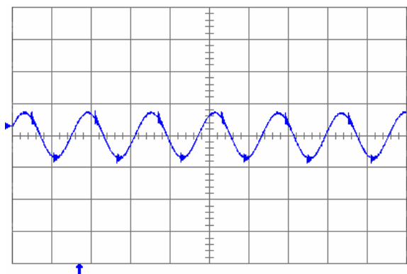
Fig. 1.5V.6: Output voltage ripple (20 mV/div.) at full rated load current into a resistive load with external capacitance 100 \mu\text{F} ceramic + 1 \mu\text{F} ceramic and V_{in} = 5 V for V_{out} = 1.5 V. Time scale: 2 \mu\text{s} /div.
