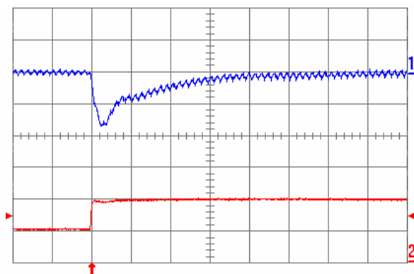
Fig. 1.5V.7: Output voltage response for V_{out} = 1.5 V to positive load current step change from 5 A to 10 A with slew rate of 5 \text{ A}/\mu\text{s} at V_{in} = 5 V. Top trace: output voltage (100 mV/div.); Bottom trace: load current (5 A/div.). C_o = 100 \mu\text{F} ceramic + 1 \mu\text{F} ceramic. Time scale: 20 \mu\text{s} /div.
