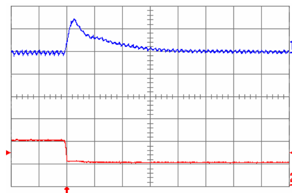
Fig. 1.0V.8: Output voltage response for V_{out} = 1.0 V to negative load current step change from 10 A to 5 A with slew rate of -5 A/ \mu s at V_{in} = 5 V. Top trace: output voltage (100 mV/div.); Bottom trace: load current (5 A/div.). C_o = 100 \mu F ceramic + 1 \mu F ceramic. Time scale: 20 \mu s/div.
