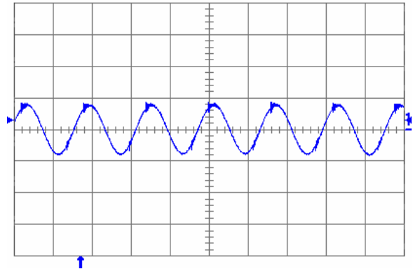
Fig. 3.3V.6: Output voltage ripple ( 20\text{ mV/div.} ) at full rated load current into a resistive load with external capacitance 100\text{ }\mu\text{F} ceramic + 1\text{ }\mu\text{F} ceramic and V_{in} = 5\text{ V} for V_{out} = 3.3\text{ V} . Time scale: 2\text{ }\mu\text{s/div.}
