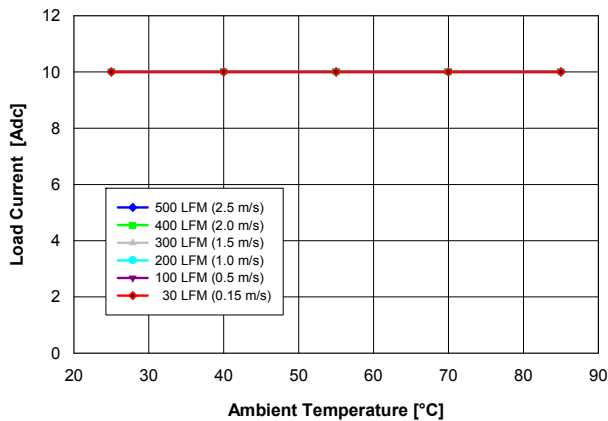
Fig. 2.0V.1: Available load current vs. ambient temperature and airflow rates for V_{out} = 2.0 V converter mounted vertically with V_{in} = 5 V, and maximum MOSFET temperature \leq 120 °C.
