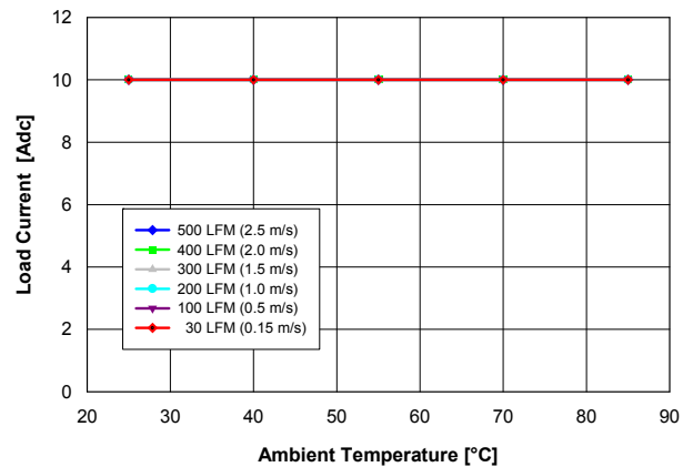
Fig. 1.0V.2: Available load current vs. ambient temperature and airflow rates for V out = 1.0 V converter mounted horizontally with V in = 5 V, and maximum MOSFET temperature ≤ 120 °C.
