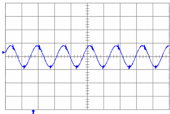
Fig. 1.8V.6: Output voltage ripple ( 20\text{ mV/div.} ) at full rated load current into a resistive load with external capacitance 100\text{ }\mu\text{F} ceramic + 1\text{ }\mu\text{F} ceramic and V_{in} = 5 V for V_{out} = 1.8 V. Time scale: 2\text{ }\mu\text{s/div.}
