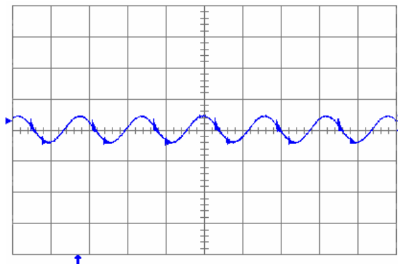
Fig. 0.7525V.6: Output voltage ripple (20 mV/div.) at full rated load current into a resistive load with external capacitance 100\text{ }\mu\text{F} ceramic + 1\text{ }\mu\text{F} ceramic and V_{in} = 5 V for V_{out} = 0.7525 V. Time scale: 2 \mu\text{s} /div.
