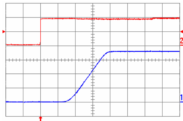
Fig. 1.8V.5: Turn-on transient for V_{out} = 1.8 V with the application of Enable signal at full rated load current (resistive) and 100\text{ }\mu\text{F} external capacitance at V_{in} = 5 V. Top trace: Enable signal ( 2\text{ V/div.} ); Bottom trace: output voltage ( 500\text{ mV/div.} ); Time scale: 2\text{ ms/div.}
