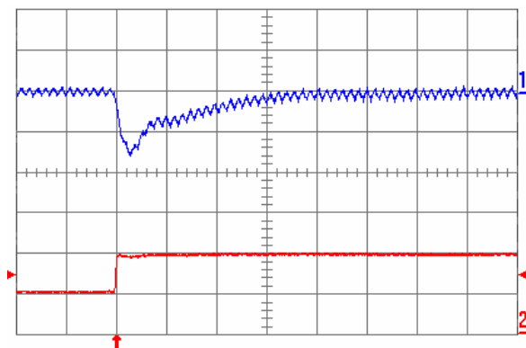
Fig. 1.8V.7: Output voltage response for V_{out} = 1.8 V to positive load current step change from 5\text{ A} to 10\text{ A} with slew rate of 5\text{ A}/\mu\text{s} at V_{in} = 5 V. Top trace: output voltage ( 100\text{ mV/div.} ); Bottom trace: load current ( 5\text{ A/div.} ). C_o = 100\text{ }\mu\text{F} ceramic + 1\text{ }\mu\text{F} ceramic. Time scale: 20\text{ }\mu\text{s/div.}
