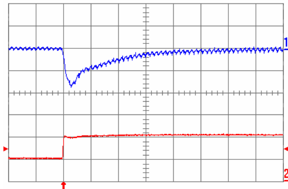
Fig. 1.2V.7: Output voltage response for V_{out} = 1.2 V to positive load current step change from 5 A to 10 A with slew rate of 5 A/ \mu s at V_{in} = 5 V. Top trace: output voltage (100 mV/div.); Bottom trace: load current (5 A/div.). C_o = 100 \mu F ceramic + 1 \mu F ceramic. Time scale: 20 \mu s/div.
