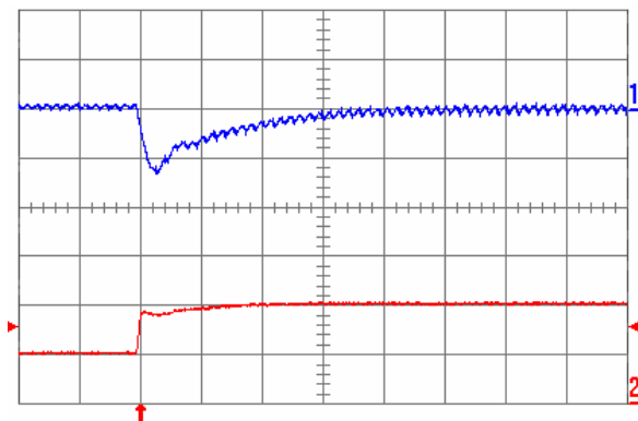
Fig. 0.7525V.7: Output voltage response for V_{out} = 0.7525 V to positive load current step change from 5 A to 10 A with slew rate of 5\text{ A}/\mu\text{s} at V_{in} = 5 V. Top trace: output voltage (100 mV/div.); Bottom trace: load current (5 A/div.). C_o = 100\text{ }\mu\text{F} ceramic + 1\text{ }\mu\text{F} ceramic. Time scale: 20 \mu\text{s} /div.
