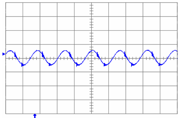
Fig. 1.0V.6: Output voltage ripple (20 mV/div.) at full rated load current into a resistive load with external capacitance 100 \mu F ceramic + 1 \mu F ceramic and V_{in} = 5 V for V_{out} = 1.0 V. Time scale: 2 \mu s/div.
