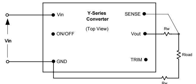
Fig. B: Remote sense circuit configuration.
