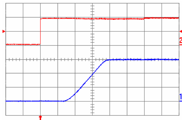
Fig. 1.5V.5: Turn-on transient for V_{out} = 1.5 V with the application of Enable signal at full rated load current (resistive) and 100 \mu\text{F} external capacitance at V_{in} = 5 V. Top trace: Enable signal (2 V/div.); Bottom trace: output voltage (500 mV/div.); Time scale: 2 ms/div.
