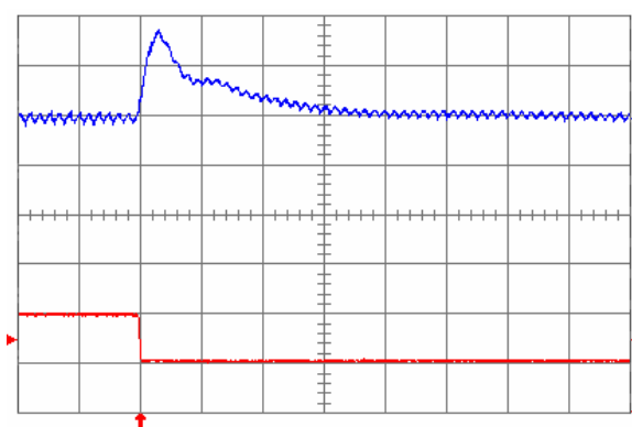
Fig. 1.5V.8: Output voltage response for V_{out} = 1.5 V to negative load current step change from 10 A to 5 A with slew rate of -5 \text{ A}/\mu\text{s} at V_{in} = 5 V. Top trace: output voltage (100 mV/div.); Bottom trace: load current (5 A/div.). C_o = 100 \mu\text{F} ceramic + 1 \mu\text{F} ceramic. Time scale: 20 \mu\text{s} /div.
