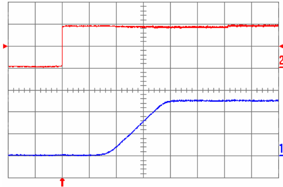
Fig. 2.5V.5: Turn-on transient for V_{out} = 2.5 V with the application of Enable signal at full rated load current (resistive) and 100 \mu\text{F} external capacitance at V_{in} = 5 V. Top trace: Enable signal (2 V/div.); Bottom trace: output voltage (1 V/div.); Time scale: 2 ms/div.
