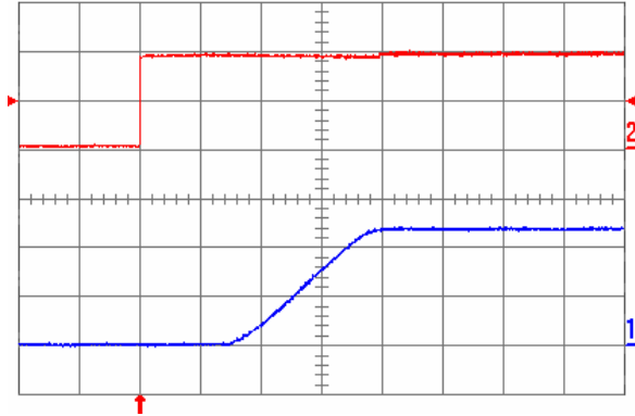
Fig. 1.2V.5: Turn-on transient for V_{out} = 1.2 V with the application of Enable signal at full rated load current (resistive) and 100 \mu F external capacitance at V_{in} = 5 V. Top trace: Enable signal (2 V/div.); Bottom trace: output voltage (500 mV/div.); Time scale: 2 ms/div.
