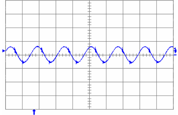
Fig. 1.2V.6: Output voltage ripple (20 mV/div.) at full rated load current into a resistive load with external capacitance 100 \mu F ceramic + 1 \mu F ceramic and V_{in} = 5 V for V_{out} = 1.2 V. Time scale: 2 \mu s/div.
