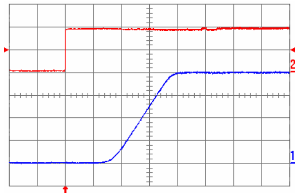
Fig. 2.0V.5: Turn-on transient for V_{out} = 2.0 V with the application of Enable signal at full rated load current (resistive) and 100 \mu F external capacitance at V_{in} = 5 V. Top trace: Enable signal (2 V/div.); Bottom trace: output voltage (500 mV/div.); Time scale: 2 ms/div.
