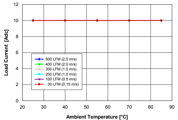
Fig. 2.0V.2: Available load current vs. ambient temperature and airflow rates for V_{out} = 2.0 V converter mounted horizontally with V_{in} = 5 V, and maximum MOSFET temperature \leq 120 °C.
