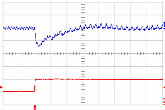
Fig. 3.3V.7: Output voltage for V_{out} = 3.3\text{ V} to positive load current step change from 5\text{ A} to 10\text{ A} with slew rate of 5\text{ A}/\mu\text{s} at V_{in} = 5\text{ V} . Top trace: output voltage ( 100\text{ mV/div.} ); Bottom trace: load current ( 5\text{ A/div.} ). C_o = 100\text{ }\mu\text{F} ceramic + 1\text{ }\mu\text{F} ceramic. Time scale: 20\text{ }\mu\text{s/div.}
