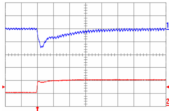
Fig. 1.0V.7: Output voltage response V_{out} = 1.0 V to positive load current step change from 5 A to 10 A with slew rate of 5 A/ \mu s at V_{in} = 5 V. Top trace: output voltage (100 mV/div.); Bottom trace: load current (5 A/div.). C_o = 100 \mu F ceramic + 1 \mu F ceramic. Time scale: 20 \mu s/div.
