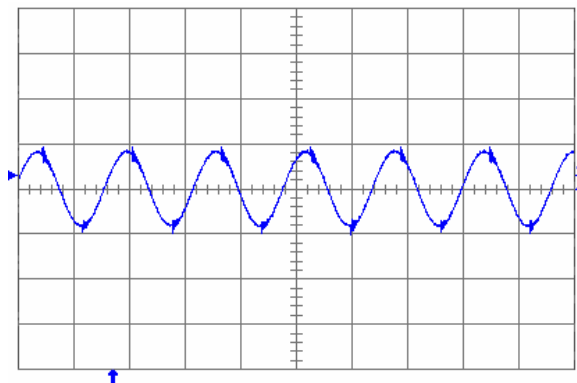
Fig. 2.0V.6: Output voltage ripple (20 mV/div.) at full rated load current into a resistive load with external capacitance 100 \mu F ceramic + 1 \mu F ceramic and V_{in} = 5 V for V_{out} = 2.0 V. Time scale: 2 \mu s/div.
