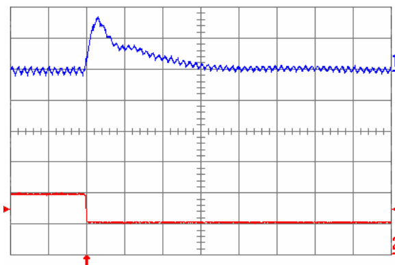
Fig. 1.8V.8: Output voltage response for V_{out} = 1.8 V to negative load current step change from 10\text{ A} to 5\text{ A} with slew rate of -5\text{ A}/\mu\text{s} at V_{in} = 5 V. Top trace: output voltage ( 100\text{ mV/div.} ); Bottom trace: load current ( 5\text{ A/div.} ). C_o = 100\text{ }\mu\text{F} ceramic + 1\text{ }\mu\text{F} ceramic. Time scale: 20\text{ }\mu\text{s/div.}
