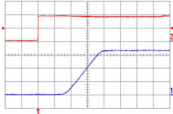
Fig. 3.3V.5: Turn-on transient for V_{out} = 3.3\text{ V} with the application of Enable signal at full rated load current (resistive) and 100\text{ }\mu\text{F} external capacitance at V_{in} = 5\text{ V} . Top trace: Enable signal ( 2\text{ V/div.} ); Bottom trace: output voltage ( 1\text{ V/div.} ); Time scale: 2\text{ ms/div.}
