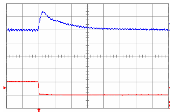
Fig. 0.7525V.8: Output voltage response for V_{out} = 0.7525 V to negative load current step change from 10 A to 8 A with slew rate of -5\text{ A}/\mu\text{s} at V_{in} = 5 V. Top trace: output voltage (100 mV/div.); Bottom trace: load current (5 A/div.). C_o = 100\text{ }\mu\text{F} ceramic + 1\text{ }\mu\text{F} ceramic. Time scale: 20 \mu\text{s} /div.
