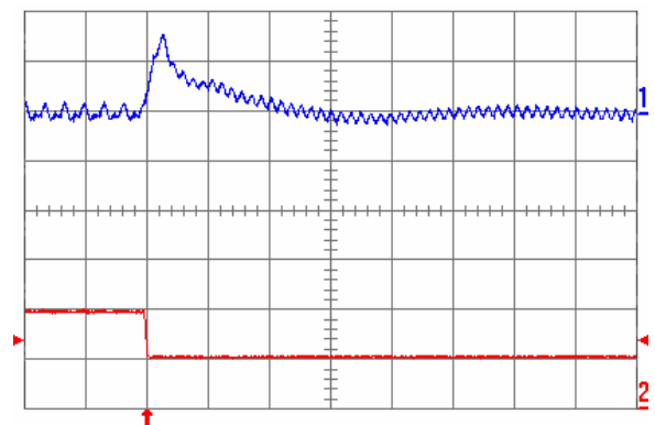
Fig. 3.3V.8: Output voltage response for V_{out} = 3.3\text{ V} to negative load current step change from 10\text{ A} to 5\text{ A} with slew rate of -5\text{ A}/\mu\text{s} at V_{in} = 5\text{ V} . Top trace: output voltage ( 100\text{ mV/div.} ); Bottom trace: load current ( 5\text{ A/div.} ). C_o = 100\text{ }\mu\text{F} ceramic + 1\text{ }\mu\text{F} ceramic. Time scale: 20\text{ }\mu\text{s/div.}
