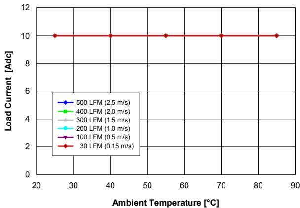
Fig. 1.0V.1: Available load current vs. ambient temperature and airflow rates for V out = 1.0 V converter mounted vertically with V in = 5 V, and maximum MOSFET temperature ≤ 120 °C.
