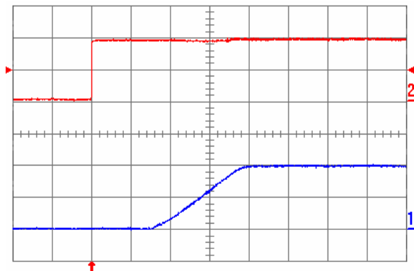
Fig. 1.0V.5: Turn-on transient for V_{out} = 1.0 V with the application of Enable signal at full rated load current (resistive) and 100 \mu F external capacitance at V_{in} = 5 V. Top trace: Enable signal (2 V/div.); Bottom trace: output voltage (500 mV/div.); Time scale: 2 ms/div.
