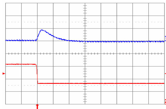
Fig. 1.5V.7: Output voltage response for V_{out} = 1.5 V to negative load current step change from 16 A to 8 A with slew rate of -5 \text{ A}/\mu\text{s} at V_{in} = 12 V. Top trace: output voltage (200 mV/div.); Bottom trace: load current (5 A/div.). C_o = 100 \mu\text{F} ceramic. Time scale: 20 \mu\text{s} /div.
