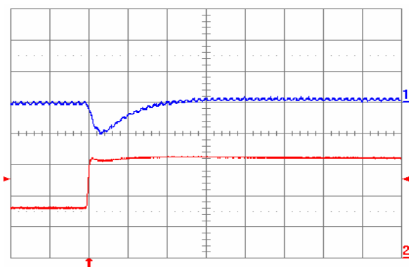
Fig. 1.8V.6: Output voltage response for V_{out} = 1.8 V to positive load current step change from 8 A to 16 A with slew rate of 5 A/ \mu s at V_{in} = 12 V. Top trace: output voltage (200 mV/div.); Bottom trace: load current (5 A/div.). C_o = 100 \mu F ceramic. Time scale: 20 \mu s/div.
