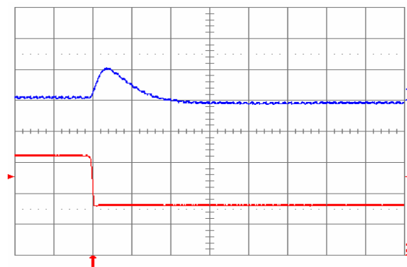
Fig. 1.2V.7: Output voltage response for V_{out} = 1.2 V to negative load current step change from 16 A to 8 A with slew rate of -5 A/ \mu s at V_{in} = 12 V. Top trace: output voltage (200 mV/div.); Bottom trace: load current (5 A/div.). C_o = 100 \mu F ceramic. Time scale: 20 \mu s/div.
