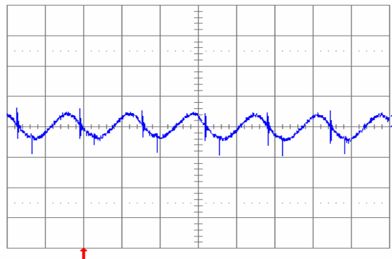
Fig. 2.5V.5: Output voltage ripple (20 mV/div.) at full rated load current into a resistive load with external capacitance 100 \mu F ceramic and V_{in} = 12 V for V_{out} = 2.5 V. Time scale: 2 \mu s/div.
