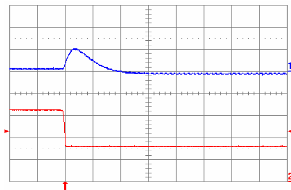
Fig. 1.0V.7: Output voltage response for V_{out} = 1.0 V to negative load current step change from 16 A to 8 A with slew rate of -5 A/ \mu s at V_{in} = 12 V. Top trace: output voltage (200 mV/div.); Bottom trace: load current (5 A/div.). C_o = 100 \mu F ceramic. Time scale: 20 \mu s/div.
