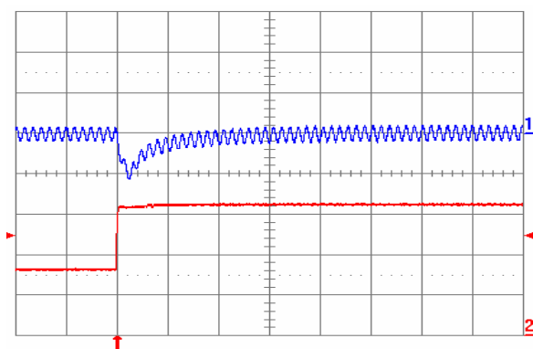
Fig. 5.0V.6: Output voltage response for V_{out} = 5.0 V to positive load current step change from 8A to 16A with slew rate of 5\ \text{A}/\mu\text{s} at V_{in} = 12 V. Top trace: output voltage (200 mV/div.); Bottom trace: load current (5 A/div.). C_o = 100\ \mu\text{F} ceramic. Time scale: 20 \mu\text{s} /div.
