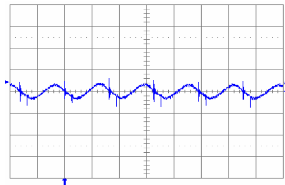
Fig. 1.8V.5: Output voltage ripple (20 mV/div.) at full rated load current into a resistive load with external capacitance 100 \mu F ceramic and V_{in} = 12 V for V_{out} = 1.8 V. Time scale: 2 \mu s/div.
