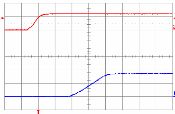
Fig. 1.8V.4: Turn-on transient for V_{out} = 1.8 V with application of V_{in} at full rated load current (resistive) and 100 \mu F external capacitance at V_{in} = 12 V. Top trace: V_{in} (10 V/div.); Bottom trace: output voltage (1 V/div.); Time scale: 2 ms/div.
