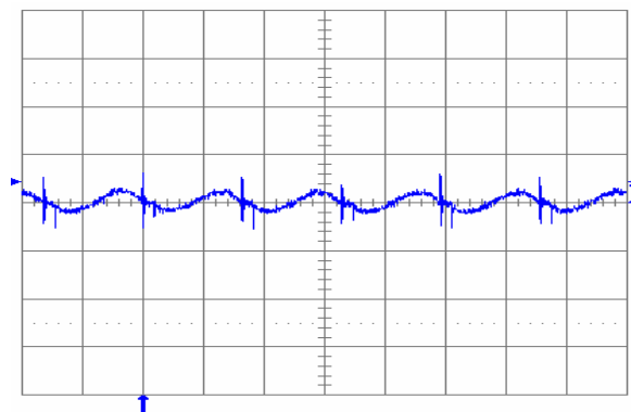
Fig. 1.2V.5: Output voltage ripple (20 mV/div.) at full rated load current into a resistive load with external capacitance 100 \mu F ceramic and V_{in} = 12 V for V_{out} = 1.2 V. Time scale: 2 \mu s/div.
