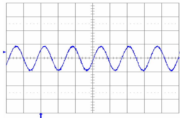
Fig. 5.0V.5: Output voltage ripple (20 mV/div.) at full rated load current into a resistive load with external capacitance 100\ \mu\text{F} ceramic and V_{in} = 12 V for V_{out} = 5.0 V. Time scale: 2 \mu\text{s} /div.
