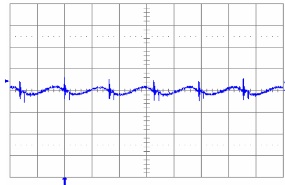
Fig. 1.0V.5: Output voltage ripple (20 mV/div.) at full rated load current into a resistive load with external capacitance 100 \mu F ceramic and V_{in} = 12 V for V_{out} = 1.0 V. Time scale: 2 \mu s/div.
