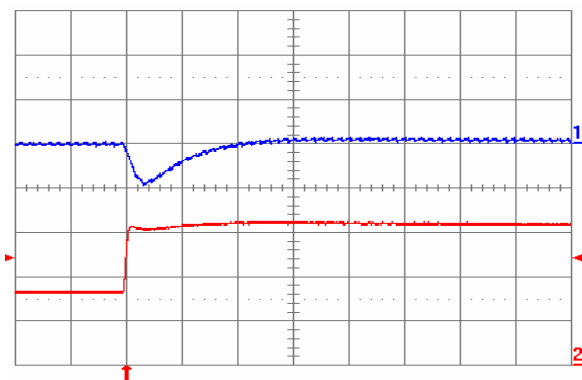
Fig. 1.5V.6: Output voltage response for V_{out} = 1.5 V to positive load current step change from 8 A to 16 A with slew rate of 5 \text{ A}/\mu\text{s} at V_{in} = 12 V. Top trace: output voltage (200 mV/div.); Bottom trace: load current (5 A/div.). C_o = 100 \mu\text{F} ceramic. Time scale: 20 \mu\text{s} /div.
