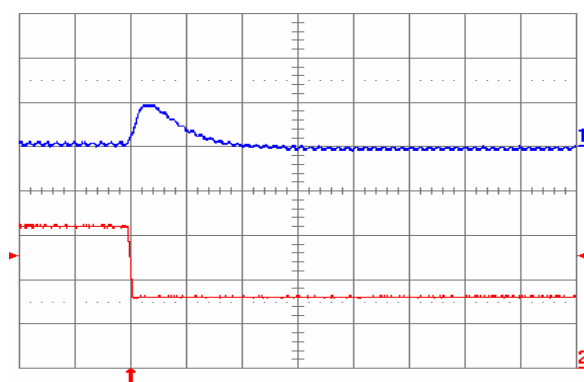
Fig. 1.8V.7: Output voltage response for V_{out} = 1.8 V to negative load current step change from 16 A to 8 A with slew rate of -5 A/ \mu s at V_{in} = 12 V. Top trace: output voltage (200 mV/div.); Bottom trace: load current (5 A/div.). C_o = 100 \mu F ceramic. Time scale: 20 \mu s/div.
