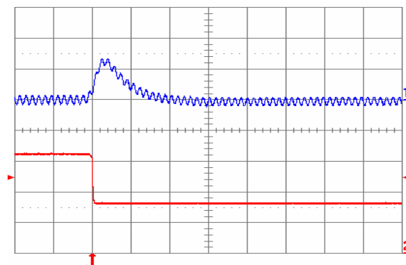
Fig. 5.0V.7: Output voltage response for V_{out} = 5.0 V to negative load current step change from 16 A to 8 A with slew rate of -5\ \text{A}/\mu\text{s} at V_{in} = 12 V. Top trace: output voltage (200 mV/div.); Bottom trace: load current (5 A/div.). C_o = 100\ \mu\text{F} ceramic. Time scale: 20 \mu\text{s} /div.
