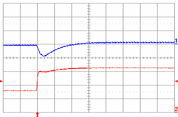
Fig. 1.0V.6: Output voltage response for V_{out} = 1.0 V to positive load current step change from 8 A to 16 A with slew rate of 5 A/ \mu s at V_{in} = 12 V. Top trace: output voltage (200 mV/div.); Bottom trace: load current (5 A/div.). C_o = 100 \mu F ceramic. Time scale: 20 \mu s/div.
