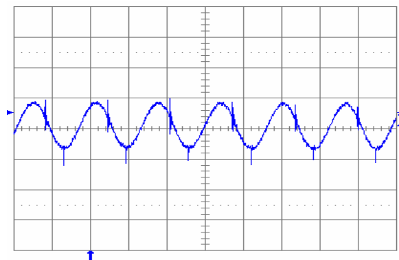
Fig. 3.3V.5: Output voltage ripple (20 mV/div.) at full rated load current into a resistive load with external capacitance 100\text{ }\mu\text{F} ceramic and V_{in} = 12\text{ V} for V_{out} = 3.3\text{ V} . Time scale: 2 \mu\text{s} /div.
