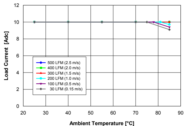
Fig. 2.5V.2: Available load current vs. ambient temperature and airflow rates for V out = 2.5V converter mounted horizontally with V in = 12V, and maximum MOSFET temperature ≤ 120°C.
