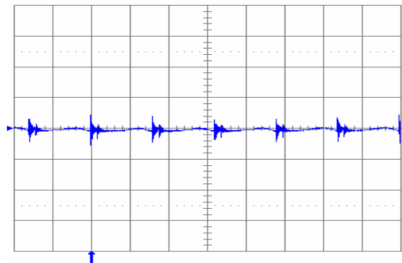
Fig. 1.2V.6: Output voltage ripple (20mV/div.) at full rated load current into a resistive load with external capacitance 100\mu F ceramic and V_{in} = 12V for V_{out} = 1.2V . Time scale: 2\mu s /div.
