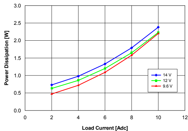
Fig. 2.0V.4: Power Loss vs. load current and input voltage for V_{out} = 2.0V converter mounted vertically with air flowing at a rate of 200 LFM (1 m/s) and T_a = 25^{\circ}C .
