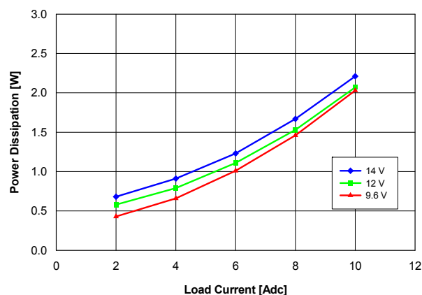
Fig. 1.5V.4: Power Loss vs. load current and input voltage for V_{out} = 1.5V converter mounted vertically with air flowing at a rate of 200 LFM (1 m/s) and T_a = 25^{\circ}C .
