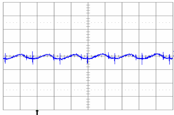
Fig. 2.5V.6: Output voltage ripple (20mV/div.) at full rated load current into a resistive load with external capacitance 100\mu F ceramic and V_{in} = 12V for V_{out} = 2.5V . Time scale: 2\mu s /div.
