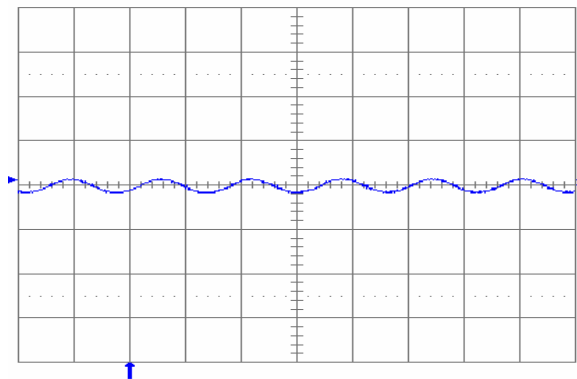
Fig. 1.8V.6: Output voltage ripple (20mV/div.) at full rated load current into a resistive load with external capacitance 100\mu F ceramic and V_{in} = 12V for V_{out} = 1.8V . Time scale: 2μs/div.
