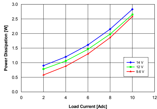
Fig. 3.3V.4: Power Loss vs. load current and input voltage for V_{out} = 3.3V converter mounted vertically with air flowing at a rate of 200 LFM (1 m/s) and T_a = 25^{\circ}C .
