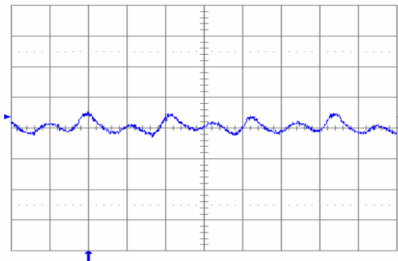
Fig. 1.5V.6: Output voltage ripple (20 mV/div.) at full rated load current into a resistive load with external capacitance 100\text{ }\mu\text{F} ceramic and V_{in} = 12\text{ V} for V_{out} = 1.5\text{ V} . Time scale: 1 \mu\text{s} /div.
