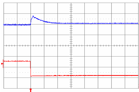
Fig. 1.8V.8: Output voltage response for V_{out} = 1.8 V to negative load current step change from 5 A to 2.5 A with slew rate of -5 A/ \mu s at V_{in} = 12 V. Top trace: output voltage (100 mV/div.); Bottom trace: load current (2 A/div.). C_o = 100 \mu F ceramic. Time scale: 20 \mu s/div.
