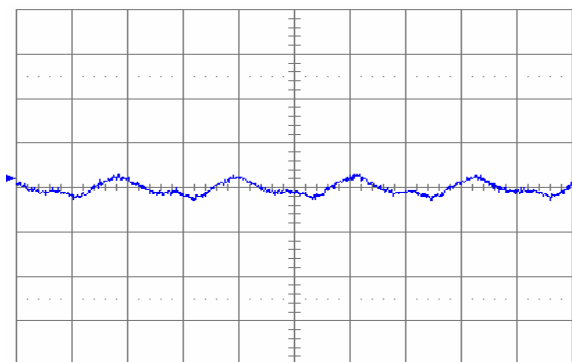
Fig. 5.0V.6: Output voltage ripple (20 mV/div.) at full rated load current into a resistive load with external capacitance 100 \mu F ceramic and V_{in} = 12 V for V_{out} = 5.0 V. Time scale: 1 \mu s/div.
