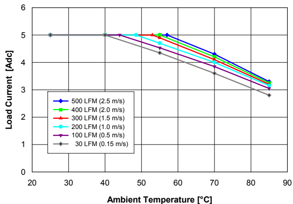
Fig. 3.3V.2: Available load current vs. ambient temperature and airflow rates for V out = 3.3 V converter mounted horizontally with V in = 12 V, and maximum MOSFET temperature ≤ 120 °C.
