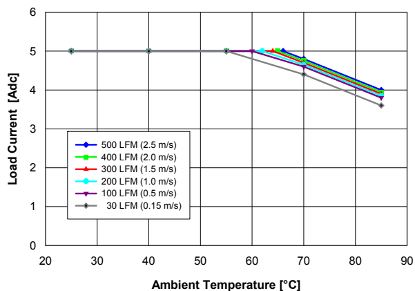
Fig. 1.0V.2: Available load current vs. ambient temperature and airflow rates for V out = 1.0 V converter mounted horizontally with V in = 12 V, and maximum MOSFET temperature ≤ 120 °C.
