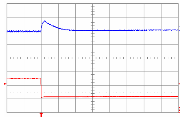
Fig. 2.0V.8: Output voltage response for V_{out} = 2.0 V to negative load current step change from 5 A to 2.5 A with slew rate of -5 A/ \mu s at V_{in} = 12 V. Top trace: output voltage (100 mV/div.); Bottom trace: load current (2 A/div.). C_o = 100 \mu F ceramic. Time scale: 20 \mu s/div.
