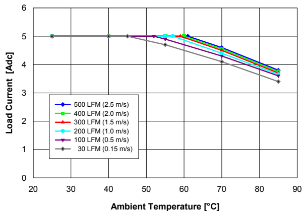
Fig. 1.5V.2: Available load current vs. ambient temperature and airflow rates for V_{out} = 1.5 V converter mounted horizontally with V_{in} = 12 V, and maximum MOSFET temperature \leq 120 °C.
