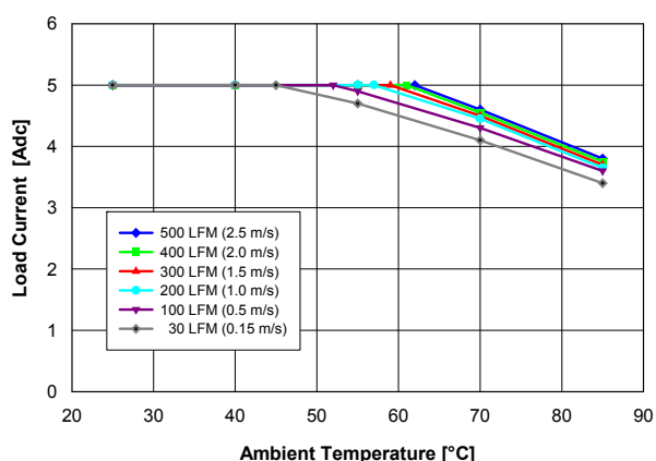
Fig. 1.8V.2: Available load current vs. ambient temperature and airflow rates for V out = 1.8 V converter mounted horizontally with V in = 12 V, and maximum MOSFET temperature ≤ 120 °C.
