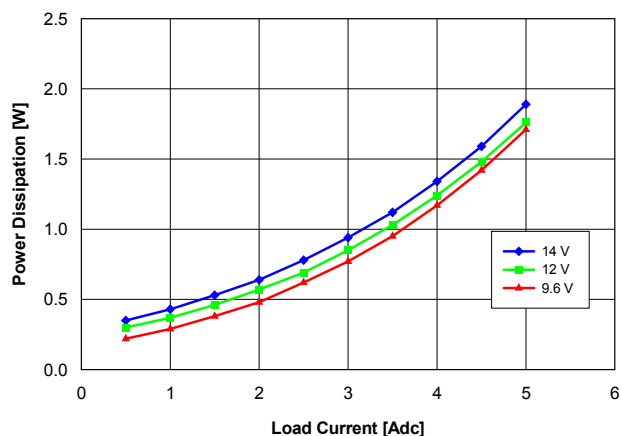
Fig. 0.7525V.4: Power Loss vs. load current and input voltage for V out = 0.7525 V converter mounted vertically with air flowing at a rate of 200 LFM (1 m/s) and T a = 25 °C.
