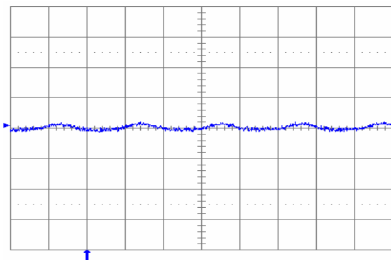
Fig. 3.3V.6: Output voltage ripple (20 mV/div.) at full rated load current into a resistive load with external capacitance 100 \mu F ceramic and V_{in} = 12 V for V_{out} = 3.3 V. Time scale: 1 \mu s/div.
