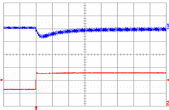
Fig. 0.7525V.7: Output voltage response for V_{out} = 0.7525\ V to positive load current step change from 2.5 A to 5 A with slew rate of 5 A/ \mu s at V_{in} = 12\ V . Top trace: output voltage (100 mV/div.); Bottom trace: load current (2 A/div.). C_o = 100\ \mu F ceramic. Time scale: 20 \mu s /div.
