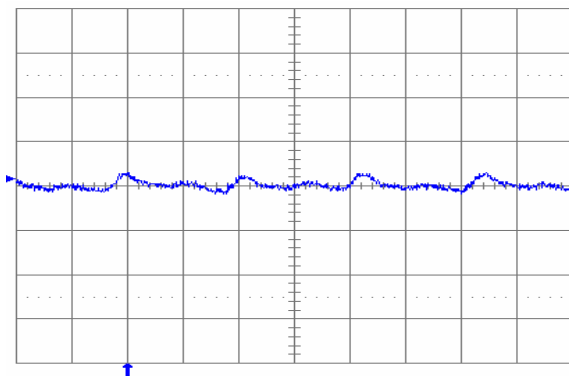
Fig. 1.0V.6: Output voltage ripple (20 mV/div.) at full rated load current into a resistive load with external capacitance 100 \mu F ceramic and V_{in} = 12 V for V_{out} = 1.0 V. Time scale: 1 \mu s/div.
