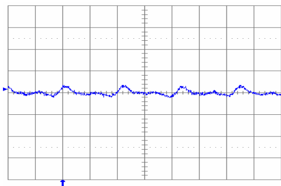
Fig. 1.8V.6: Output voltage ripple (20 mV/div.) at full rated load current into a resistive load with external capacitance 100 \mu F ceramic and V_{in} = 12 V for V_{out} = 1.8 V. Time scale: 1 \mu s/div.
