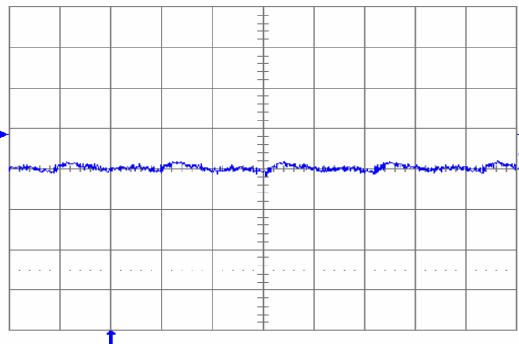
Fig. 0.7525V.6: Output voltage ripple (20 mV/div.) at full rated load current into a resistive load with external capacitance 100\ \mu F ceramic and V_{in} = 12\ V for V_{out} = 0.7525\ V . Time scale: 1 \mu s /div.
