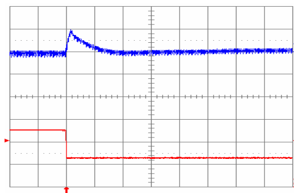
Fig. 5.0V.8: Output voltage response for V_{out} = 5.0 V to negative load current step change from 5 A to 2.5 A with slew rate of -5A/ \mu s at V_{in} = 12 V. Top trace: output voltage (100 mV/div.); Bottom trace: load current (2 A/div.). C_o = 100\mu F ceramic. Time scale: 20 \mu s/div.
