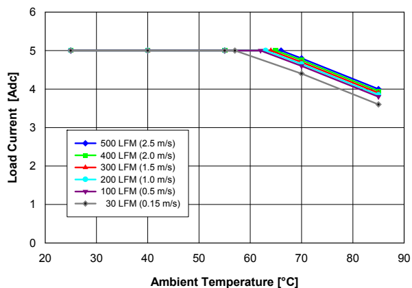
Fig. 1.2V.2: Available load current vs. ambient temperature and airflow rates for V out = 1.2 V converter mounted horizontally with V in = 12 V, and maximum MOSFET temperature ≤ 120 °C.
