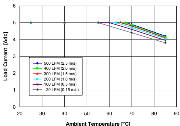
Fig. 0.7525V.2: Available load current vs. ambient temperature and airflow rates for V out = 0.7525 V converter mounted horizontally with V in = 12 V, and maximum MOSFET temperature ≤ 120 °C.
