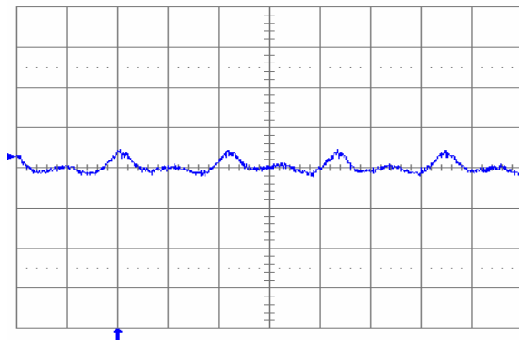
Fig. 2.5V.6: Output voltage ripple (20 mV/div.) at full rated load current into a resistive load with external capacitance 100 \mu F ceramic + 1 \mu F ceramic and V_{in} = 12 V for V_{out} = 2.5 V. Time scale: 2 \mu s/div.
