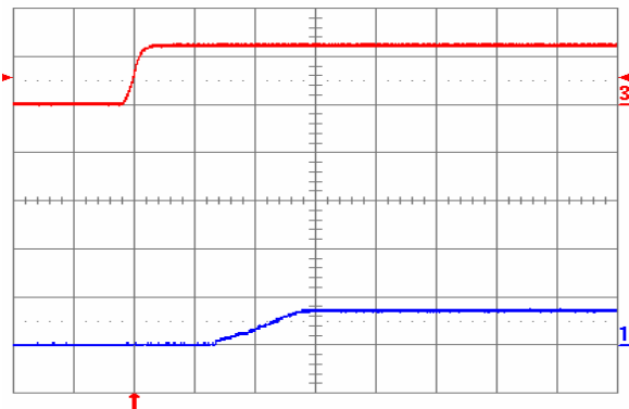
Fig. 0.7525V.5: Turn-on transient for V_{out} = 0.7525V with application of V_{in} at full rated load current (resistive) and 100\ \mu F external capacitance at V_{in} = 12\ V . Top trace: V_{in} (10 V/div.); Bottom trace: output voltage (1 V/div.); Time scale: 5 ms/div.
