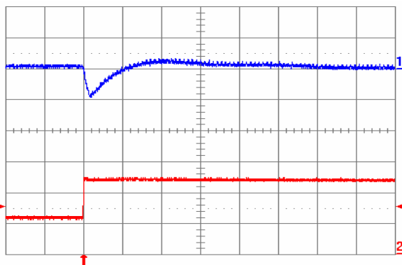
Fig. 3.3V.7: Output voltage response for V_{out} = 3.3 V to positive load current step change from 2.5 A to 5 A with slew rate of 5 A/ \mu s at V_{in} = 12 V. Top trace: output voltage (100 mV/div.); Bottom trace: load current (2 A/div.). C_o = 100 \mu F ceramic. Time scale: 20 \mu s/div.
