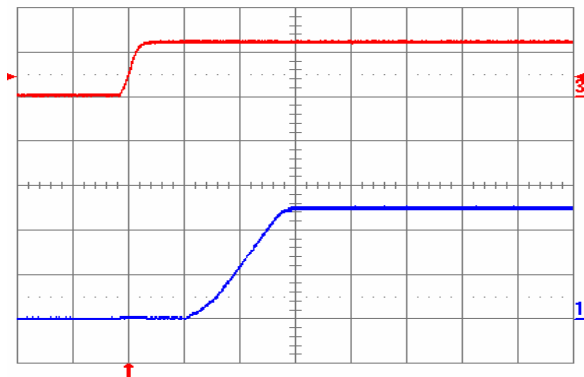
Fig. 2.5V.5: Turn-on transient for V_{out} = 2.5 V with application of V_{in} at full rated load current (resistive) and 100 \mu F external capacitance at V_{in} = 12 V. Top trace: V_{in} (10 V/div.); Bottom trace: output voltage (1 V/div.); Time scale: 5 ms/div.
