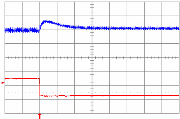
Fig. 1.5V.8: Output voltage response for V_{out} = 1.5\text{ V} to negative load current step change from 5 A to 2.5 A with slew rate of -5\text{ A}/\mu\text{s} at V_{in} = 12\text{ V} . Top trace: output voltage (100 mV/div.); Bottom trace: load current (2 A/div.). C_o = 100\text{ }\mu\text{F} ceramic. Time scale: 20 \mu\text{s} /div.
