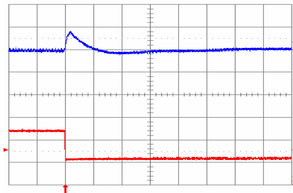
Fig. 3.3V.8: Output voltage response for V_{out} = 3.3 V to negative load current step change from 5 A to 2.5 A with slew rate of -5 A/ \mu s at V_{in} = 12 V. Top trace: output voltage (100 mV/div.); Bottom trace: load current (2 A/div.). C_o = 100 \mu F ceramic. Time scale: 20 \mu s/div.
