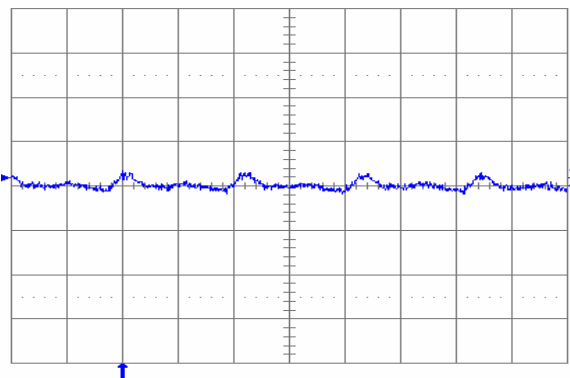
Fig. 1.2V.6: Output voltage ripple (20 mV/div.) at full rated load current into a resistive load with external capacitance 100 \mu F ceramic and V_{in} = 12 V for V_{out} = 1.2 V. Time scale: 1 \mu s/div.
