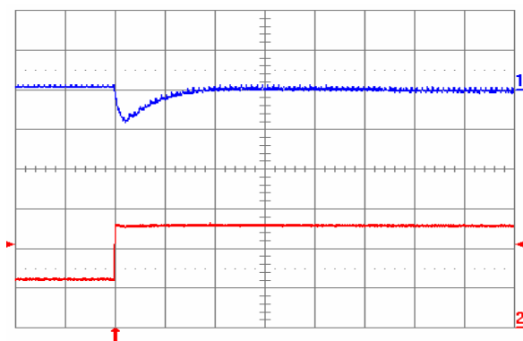
Fig. 2.0V.7: Output voltage response for V_{out} = 2.0 V to positive load current step change from 2.5 A to 5 A with slew rate of 5 A/ \mu s at V_{in} = 12 V. Top trace: output voltage (100 mV/div.); Bottom trace: load current (2 A/div.). C_o = 100 \mu F ceramic. Time scale: 20 \mu s/div.
