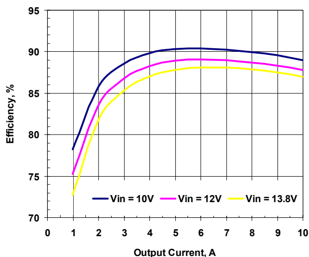
Figure 3. Efficiency vs. Load. Vout=2.5
