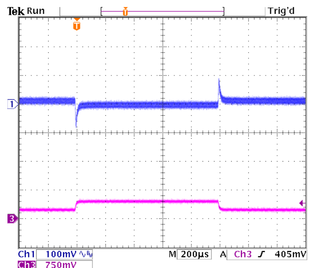
Figure 13. Transient Response to Dynamic Load Change from 50% to 100% of full load (Vin=12V, Vo=5.0Vdc). Ch3 – Iout. Scale=10A/div
