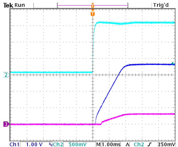
Figure 8. Typical Start-Up Using Remote On/Off (Vo = 3.3 Vdc, Io=6A). Ch1 – Vout, Ch2 – ON/OFF, Ch3 – Iout. Scale=10A/div
