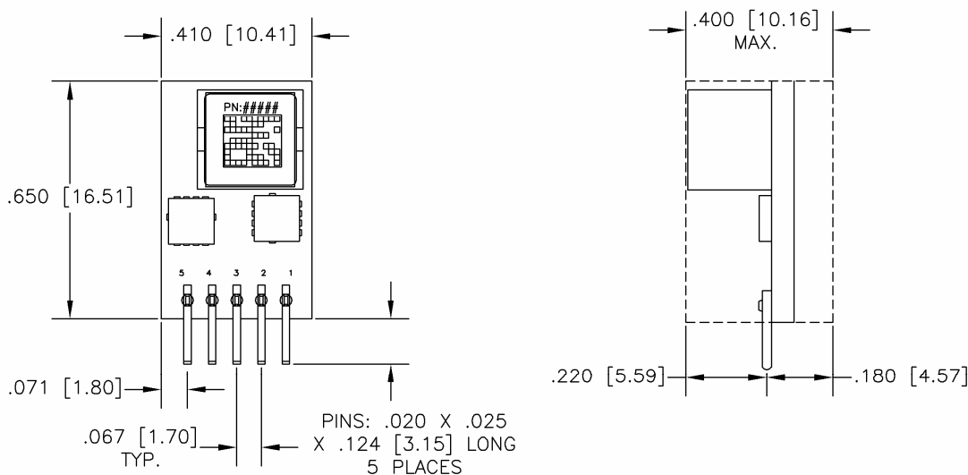
Figure 17. Mechanical Drawing
