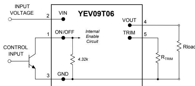
Figure 15. Circuit Configuration For ON/OFF Function
