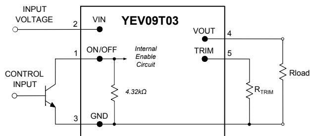
Figure 13. Circuit Configuration For ON/OFF Function
