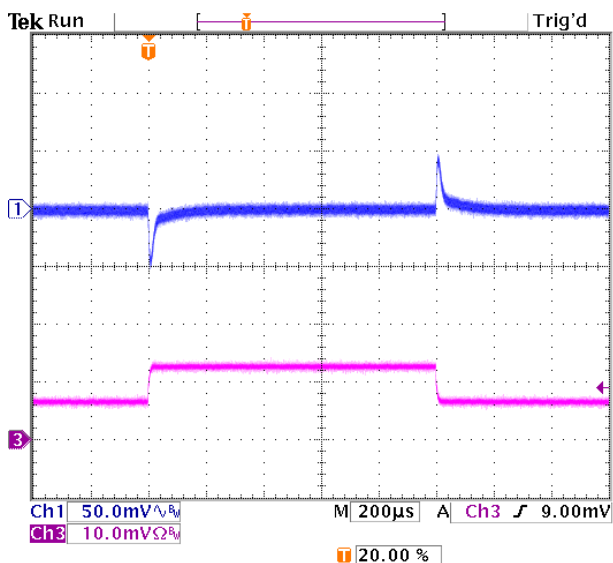
Figure 11. Transient Response to Dynamic Load Change from 40% to 80% of full load ( V_{in}=12V , V_o=3.3Vdc ). Ch3 – Iout. Scale=0.2A/mV
