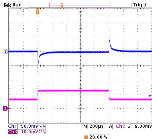
Figure 9. Transient Response to Dynamic Load Change from 40% to 80% of full load (Vin=12V, Vo=1.2Vdc). Ch3 – Iout. Scale=0.2A/mV
