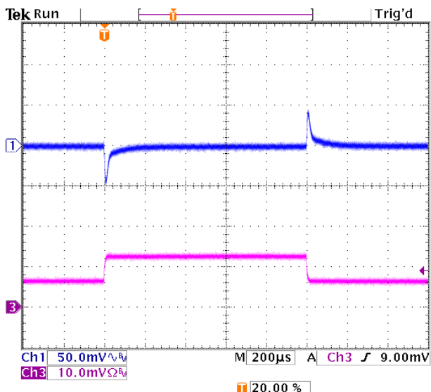
Figure 10. Transient Response to Dynamic Load Change from 40% to 80% of full load ( V_{in}=12V , V_o=2.5Vdc ). Ch3 – Iout. Scale=0.2A/mV
