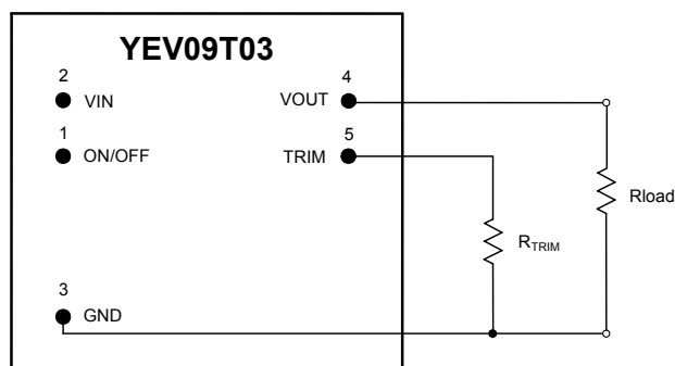
Figure 12. Programming Output Voltage With A Resistor
