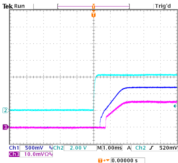
Figure 5. Typical Start-Up Using Remote On/Off (Vo = 1.2 Vdc, Io=3A). Ch1 – Vout, Ch2 – ON/OFF, Ch3 – Iout
