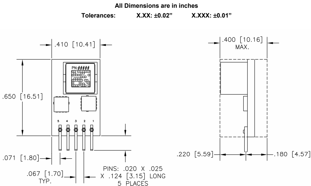
Figure 15. Mechanical Drawing
