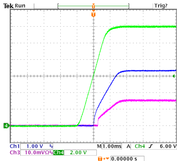
Figure 8. Typical Start-Up with application of Vin (Vo = 3.3Vdc, Io = 3A). Ch1 – Vout, Ch3 – Iout, Ch4 – Vin,
