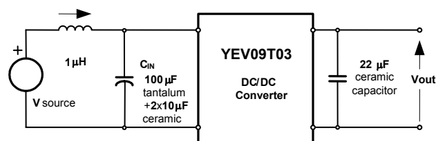
Figure 14. Test Setup For Measuring Input Reflected-Ripple Current And Output Voltage Ripple
