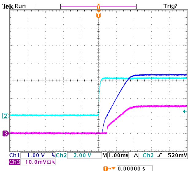
Figure 6. Typical Start-Up Using Remote On/Off (Vo = 3.3 Vdc, Io=3A). Ch1 – Vout, Ch2 – ON/OFF, Ch3 – Iout
