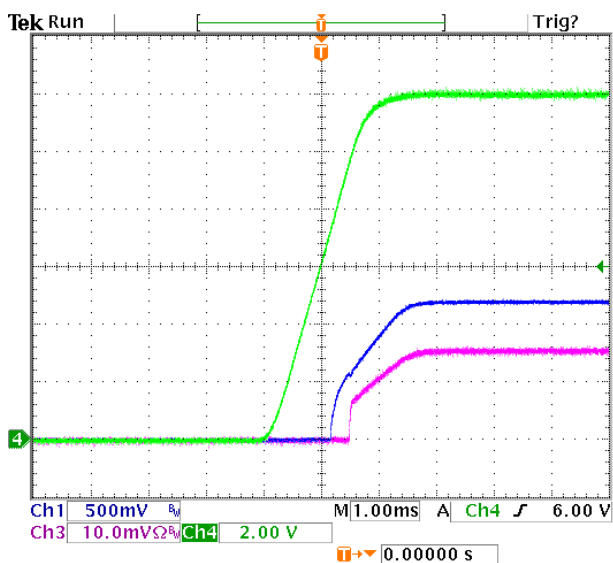
Figure 7. Typical Start-Up with application of Vin (Vo = 1.2Vdc, Io = 3A). Ch1 – Vout, Ch3 – Iout, Ch4 – Vin.
