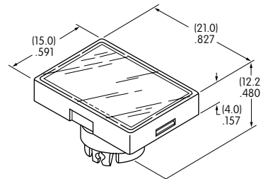
AT3016 Rectangular
