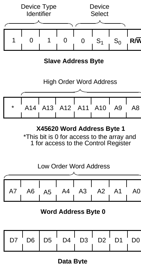
Figure 10. Device Addressing
