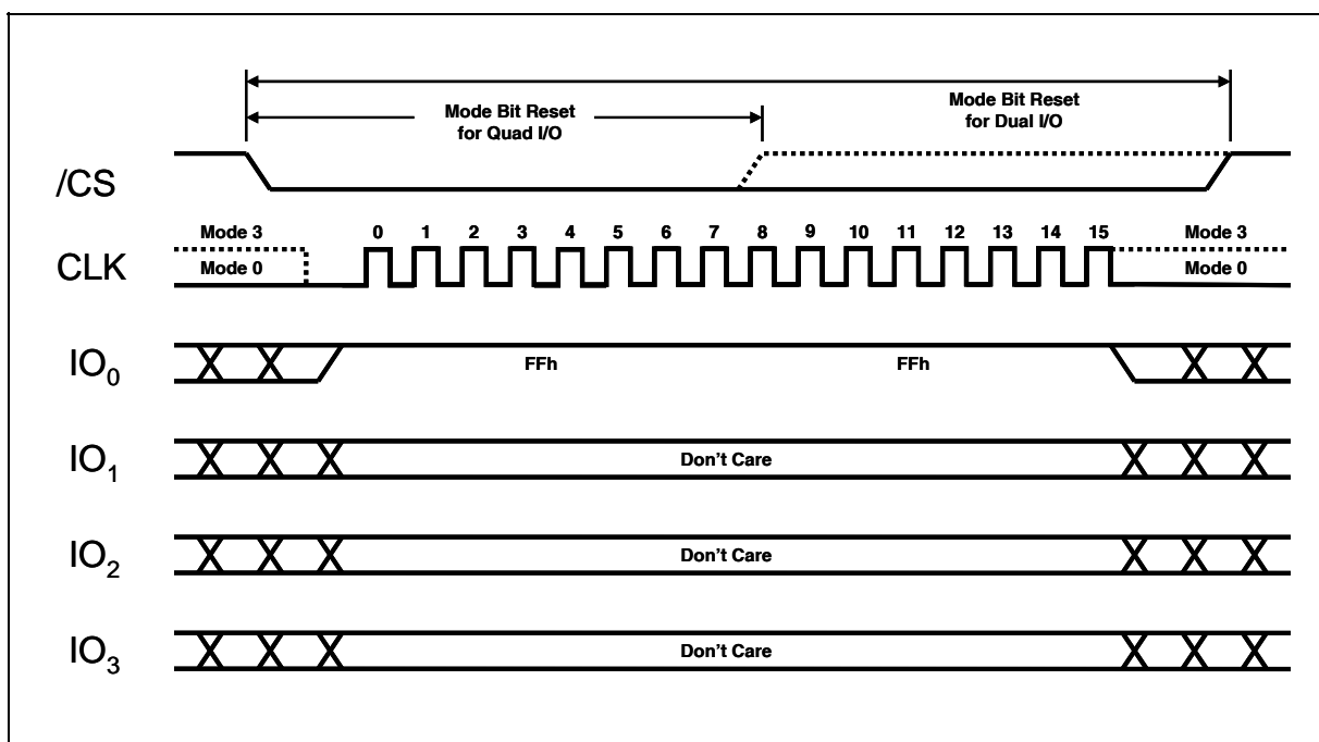
Figure 30. Continuous Read Mode Reset for Fast Read Dual/Quad I/O
