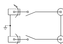
NON-NORMALLED NON-TERMINATED
