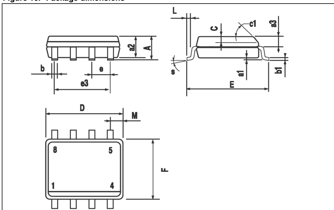
Figure 10. Package dimensions
