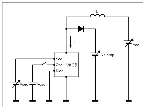
Test circuit
