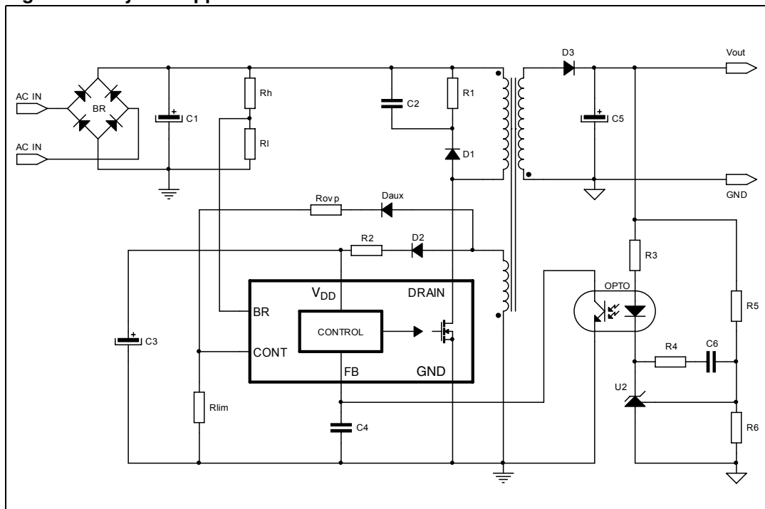
Figure 21. Flyback application
