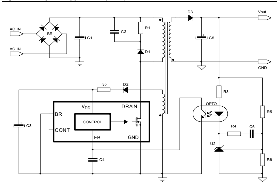
Figure 20. Flyback application (basic)
