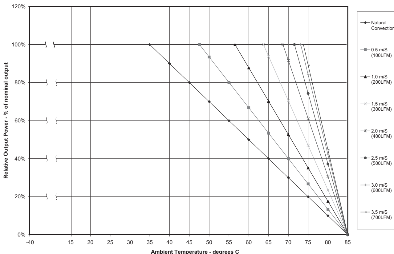
FIGURE 1b. OUTPUT DERATING (48 V)
