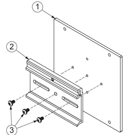
ASSEMBLY DRAWING
