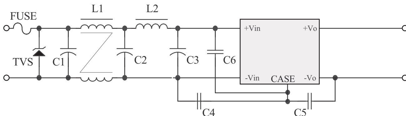
FIGURE 10.2. EMI FILTER FOR VHB50W, 48 V
