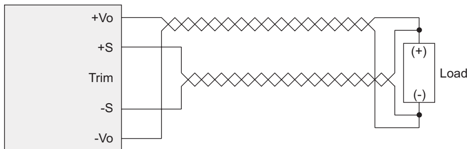
FIGURE 2. REMOTE SENSE
