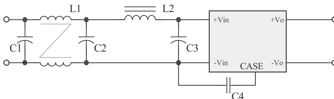
FIGURE 10.1. EMI FILTER FOR VHB50W, 3.3 ~ 24 V
