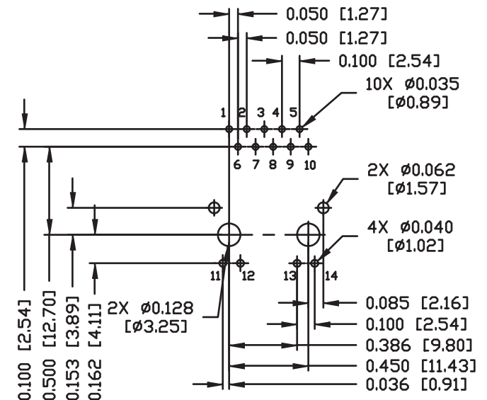
RECOMMENDED PCB FOOTPRINT COMPONENT SIDE VIEW
