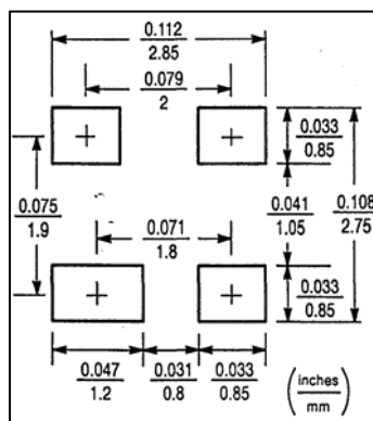
PAD LAYOUT
