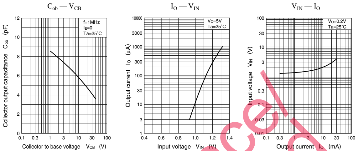
Characteristics charts of UNR1224
