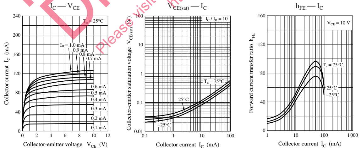
Characteristics charts of UNR1218
