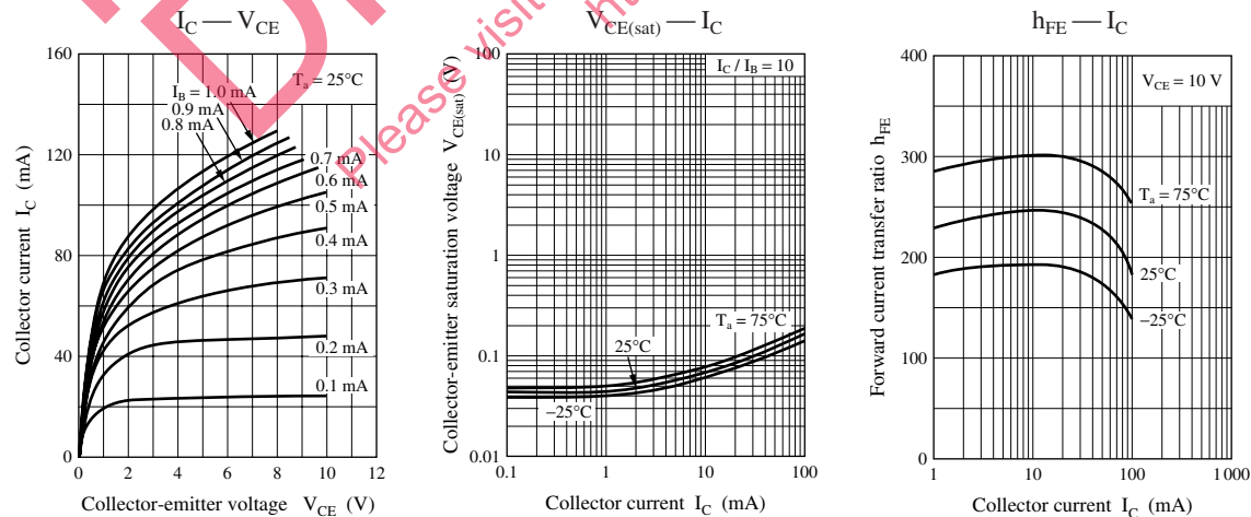
Characteristics charts of UNR1215
