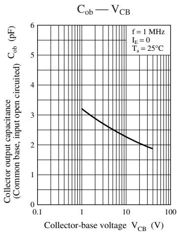
Characteristics charts of UNR1213
