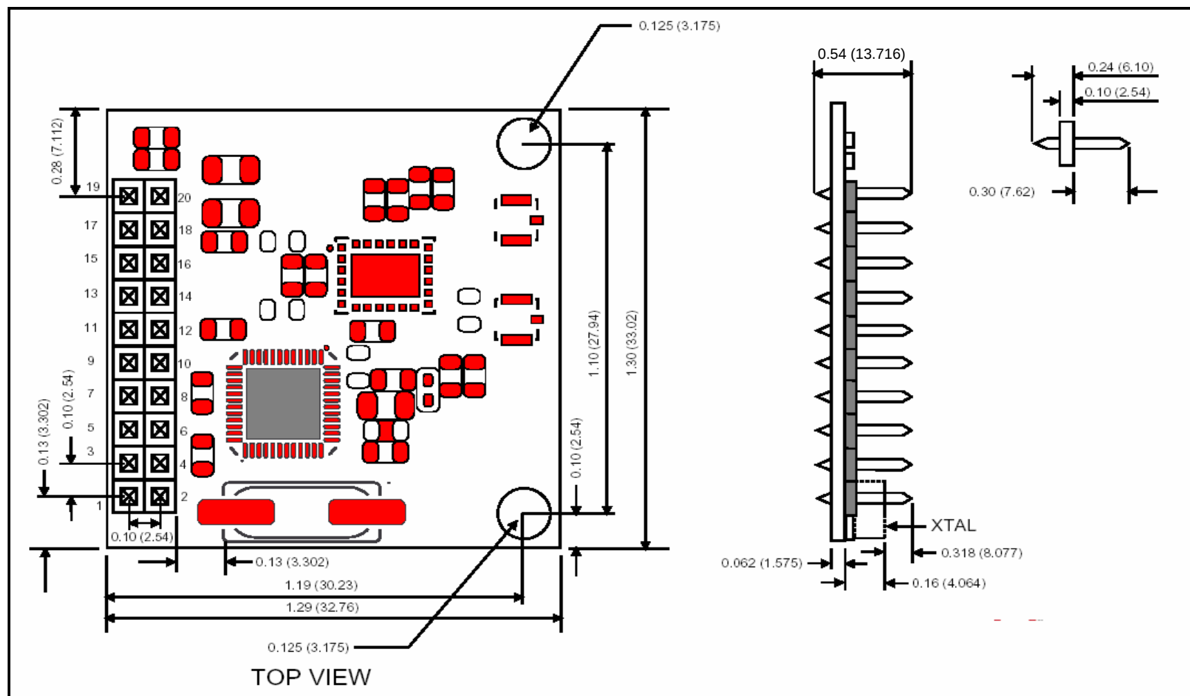
Figure 4 – Juno-LPA Dimensions
