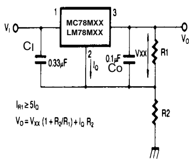
Figure 3. Circuit for Increasing Output Voltage
