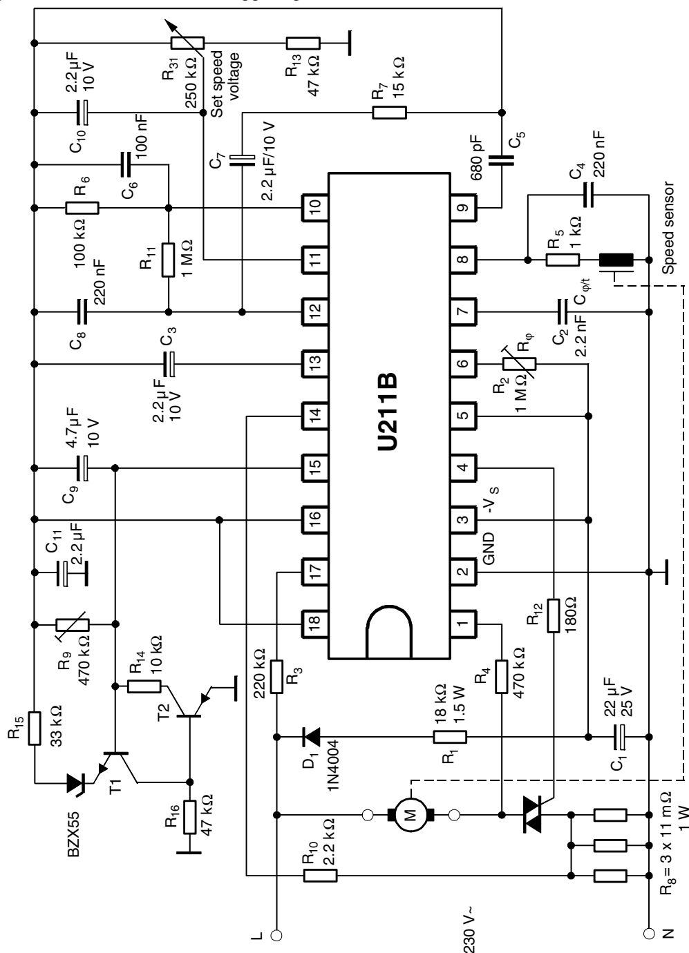
Figure 10-19. Speed Control, Automatic Retriggering, Load Switch-down, Soft Start
