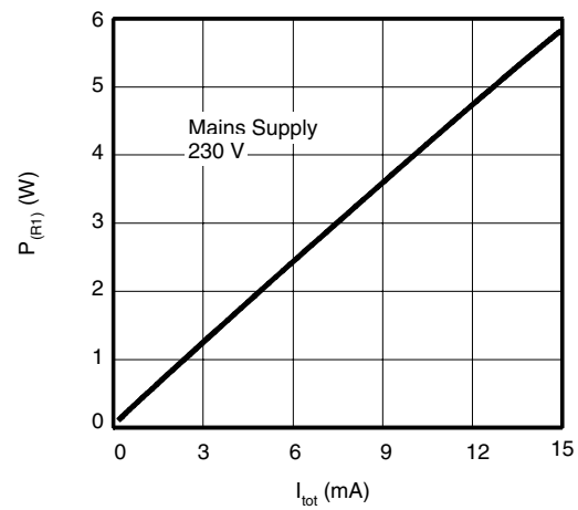
Figure 10-16. Power Dissipation of R_1 According to Current Consumption
