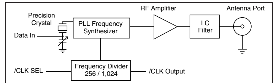
Figure 8: ES Series Transmitter Block Diagram
