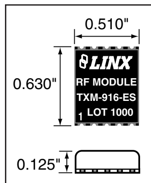
Figure 1: Package Dimensions
