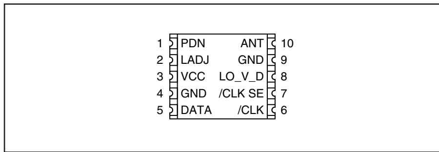
Figure 7: ES Series Transmitter Pinout (Top View)
