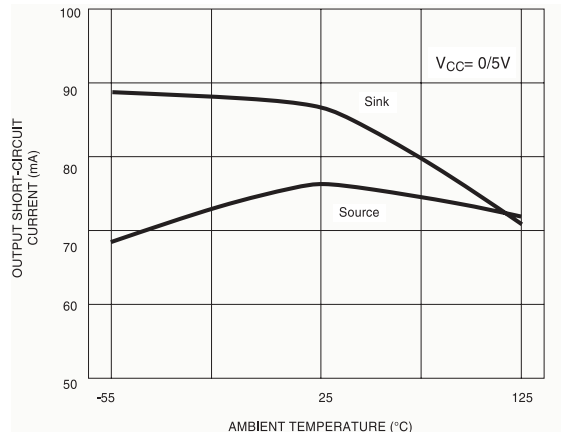
Figure 7. Output short circuit current vs. temperature
