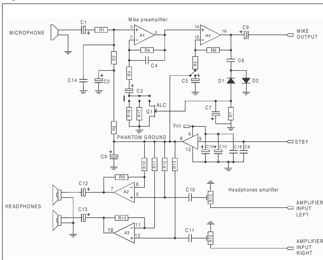
Figure 16. Electrical schematic
