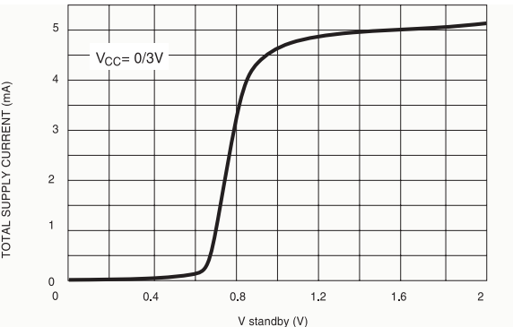
Figure 14. Total supply current vs. standby input voltage
