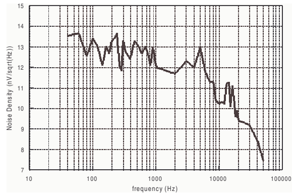
Figure 18. Voltage noise density vs. frequency at preamplifier output
