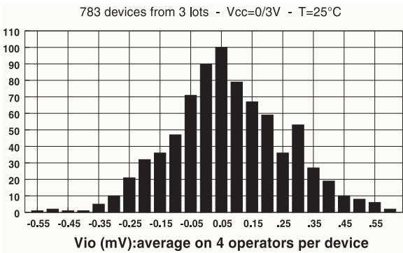
Figure 1. Input offset voltage distribution
